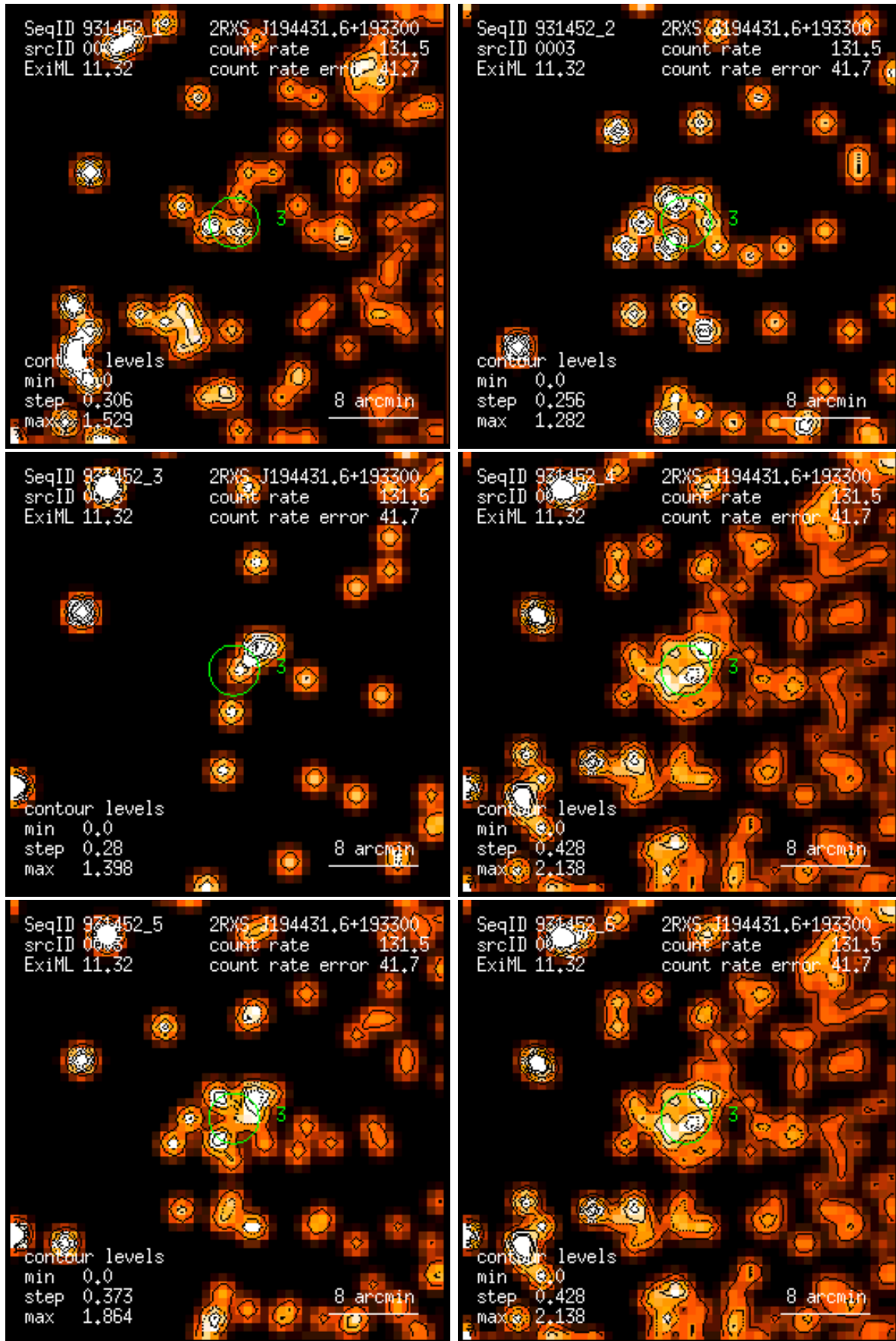
Figure 3: RASS 931452: detection 0003: band rate images, Gaussian filter: (1) PSPC channels 11 – 41, (2) 52 – 90, (3) 91 – 201, (4) 11 – 235, (5) 52 – 201, (6) 11 – 201. Broad band rates in counts/ks. Band rate contour levels in counts/ks/arcmin 2 .
