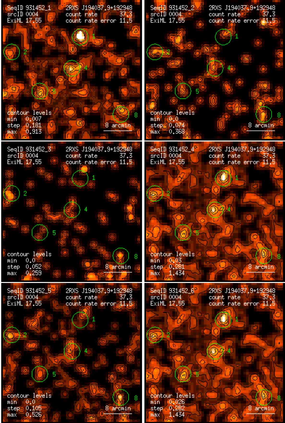
Figure 4: RASS 931452: detection 0004: band rate images, Gaussian filter: (1) PSPC channels 11 – 41, (2) 52 – 90, (3) 91 – 201, (4) 11 – 235, (5) 52 – 201, (6) 11 – 201. Broad band rates in counts/ks. Band rate contour levels in counts/ks/arcmin 2 .
