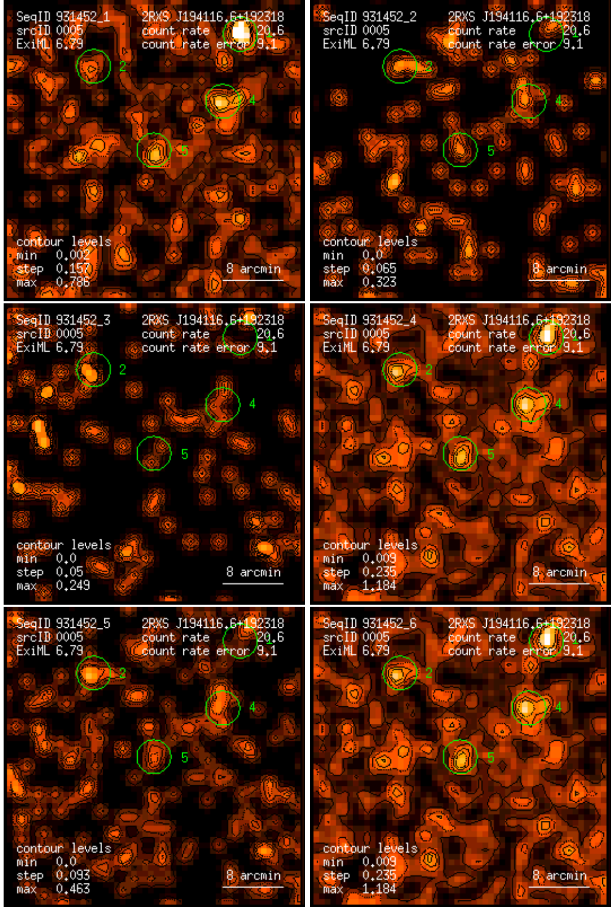
Figure 5: RASS 931452: detection 0005: band rate images, Gaussian filter: (1) PSPC channels 11 – 41, (2) 52 – 90, (3) 91 – 201, (4) 11 – 235, (5) 52 – 201, (6) 11 – 201. Broad band rates in counts/ks. Band rate contour levels in counts/ks/arcmin 2 .
