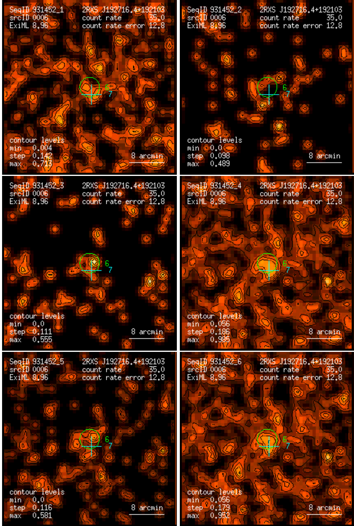
Figure 6: RASS 931452: detection 0006: band rate images, Gaussian filter: (1) PSPC channels 11 – 41, (2) 52 – 90, (3) 91 – 201, (4) 11 – 235, (5) 52 – 201, (6) 11 – 201. Broad band rates in counts/ks. Band rate contour levels in counts/ks/arcmin 2 .
