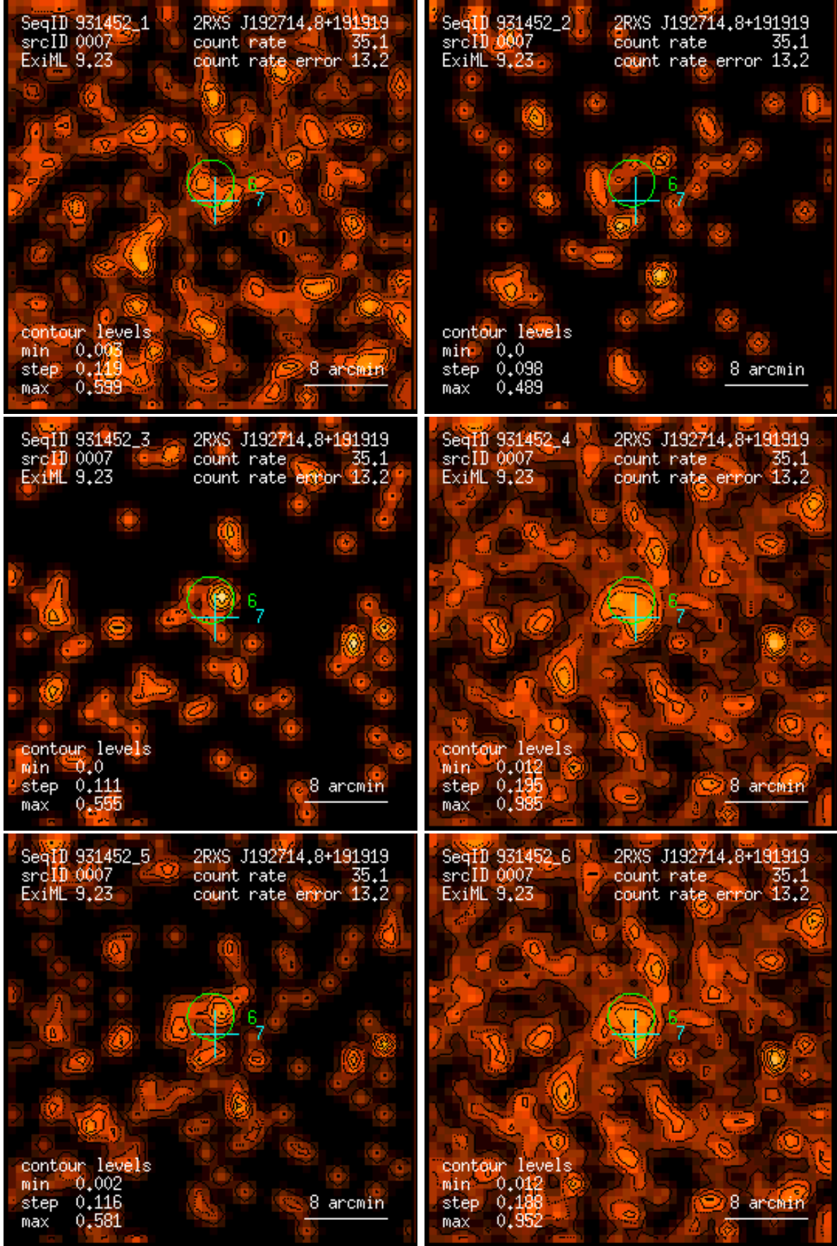
Figure 7: RASS 931452: detection 0007: band rate images, Gaussian filter: (1) PSPC channels 11 – 41, (2) 52 – 90, (3) 91 – 201, (4) 11 – 235, (5) 52 – 201, (6) 11 – 201. Broad band rates in counts/ks. Band rate contour levels in counts/ks/arcmin 2 .
