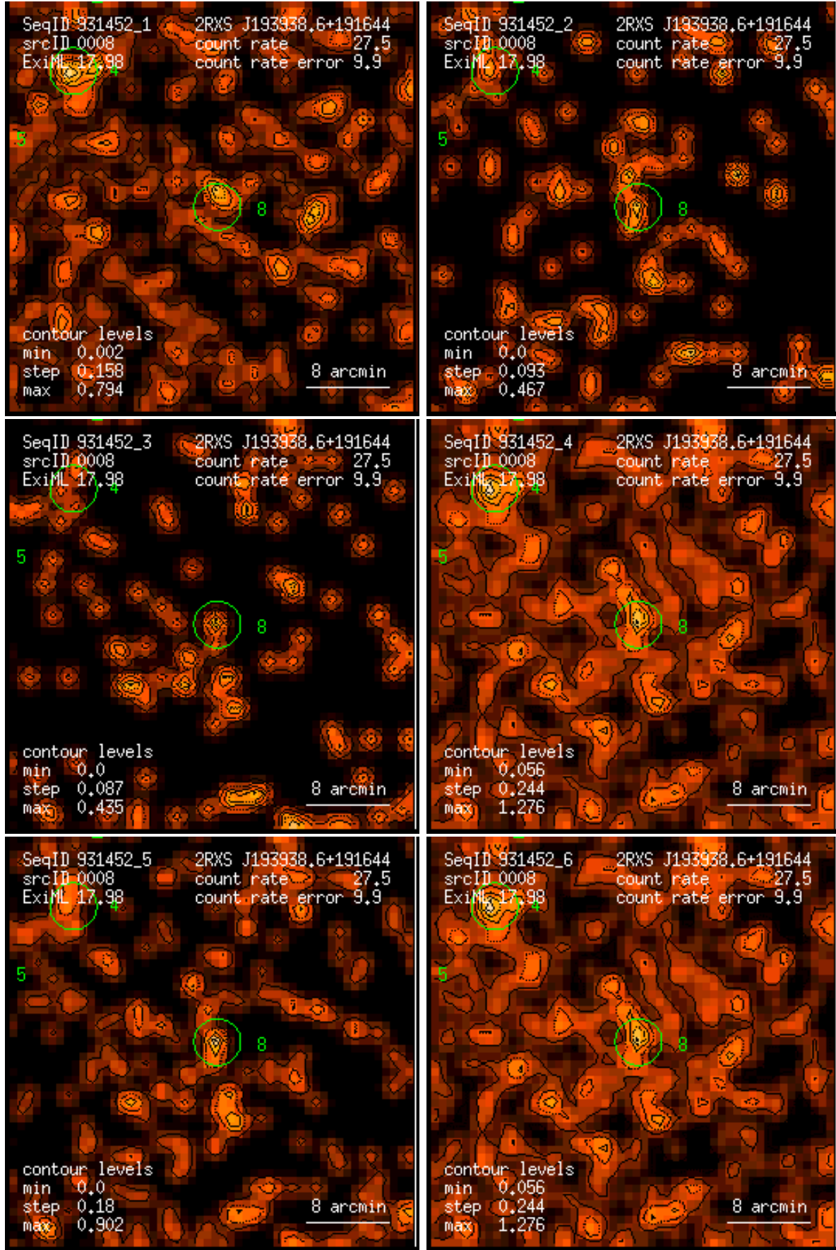
Figure 8: RASS 931452: detection 0008: band rate images, Gaussian filter: (1) PSPC channels 11 – 41, (2) 52 – 90, (3) 91 – 201, (4) 11 – 235, (5) 52 – 201, (6) 11 – 201. Broad band rates in counts/ks. Band rate contour levels in counts/ks/arcmin 2 .
