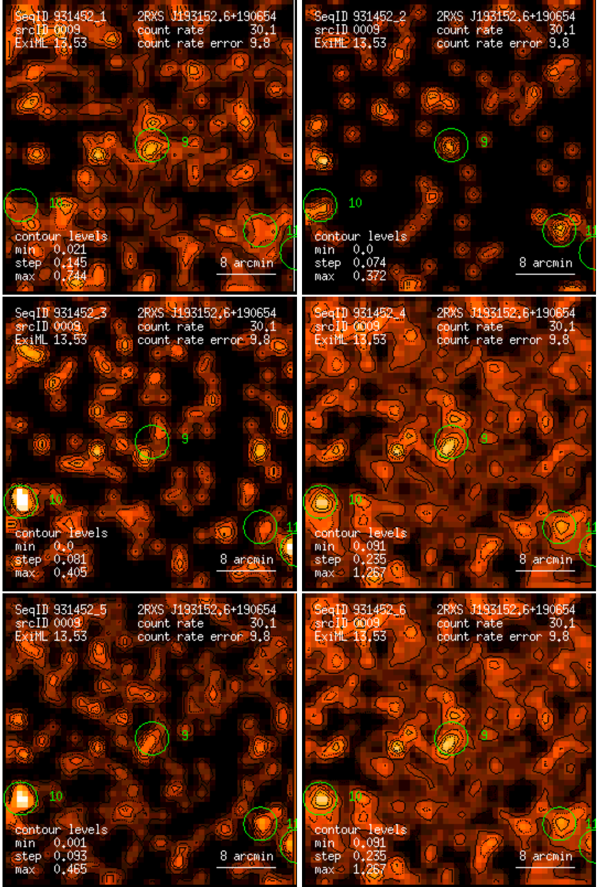
Figure 9: RASS 931452: detection 0009: band rate images, Gaussian filter: (1) PSPC channels 11 – 41, (2) 52 – 90, (3) 91 – 201, (4) 11 – 235, (5) 52 – 201, (6) 11 – 201. Broad band rates in counts/ks. Band rate contour levels in counts/ks/arcmin 2 .
