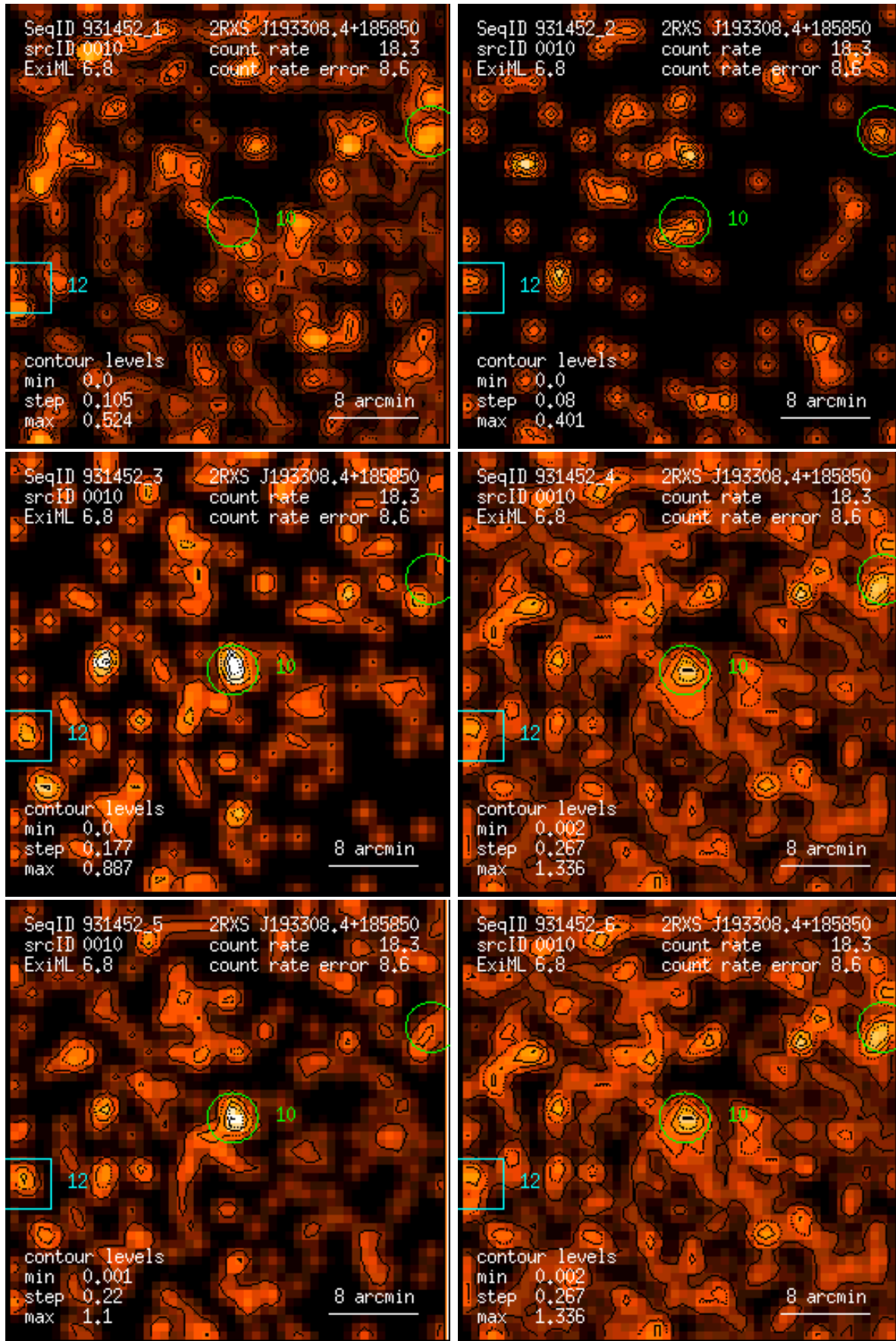
Figure 10: RASS 931452: detection 0010: band rate images, Gaussian filter: (1) PSPC channels 11 – 41, (2) 52 – 90, (3) 91 – 201, (4) 11 – 235, (5) 52 – 201, (6) 11 – 201. Broad band rates in counts/ks. Band rate contour levels in counts/ks/arcmin 2 .
