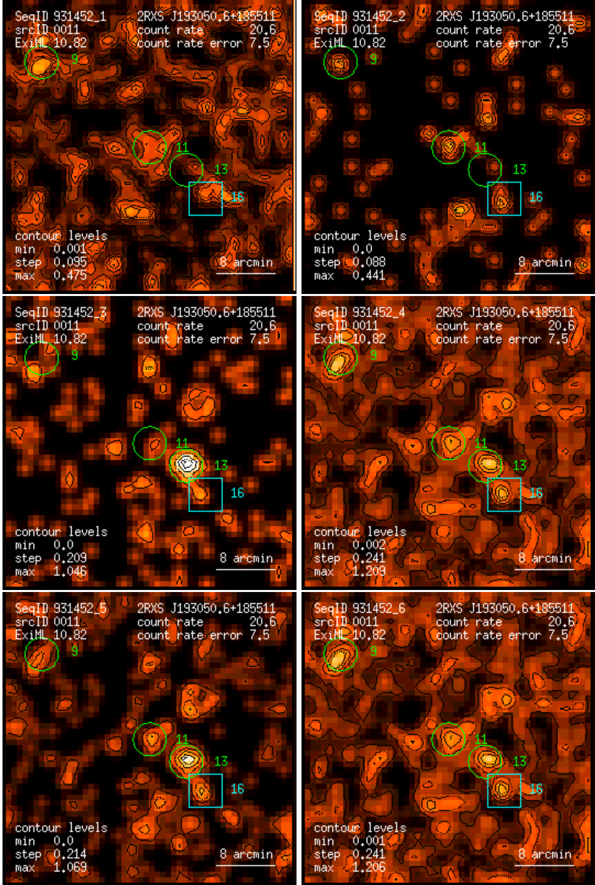
Figure 11: RASS 931452: detection 0011: band rate images, Gaussian filter: (1) PSPC channels 11 – 41, (2) 52 – 90, (3) 91 – 201, (4) 11 – 235, (5) 52 – 201, (6) 11 – 201. Broad band rates in counts/ks. Band rate contour levels in counts/ks/arcmin 2 .
