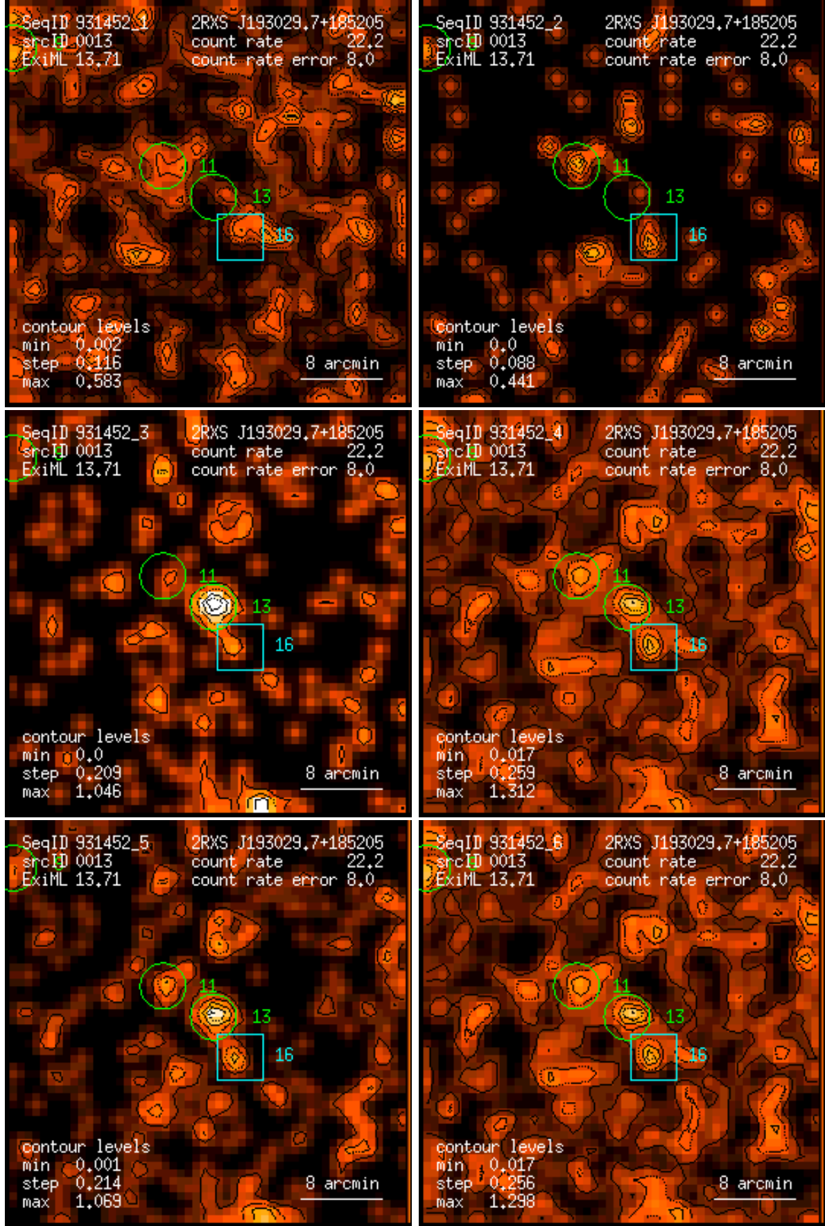
Figure 13: RASS 931452: detection 0013: band rate images, Gaussian filter: (1) PSPC channels 11 – 41, (2) 52 – 90, (3) 91 – 201, (4) 11 – 235, (5) 52 – 201, (6) 11 – 201. Broad band rates in counts/ks. Band rate contour levels in counts/ks/arcmin 2 .
