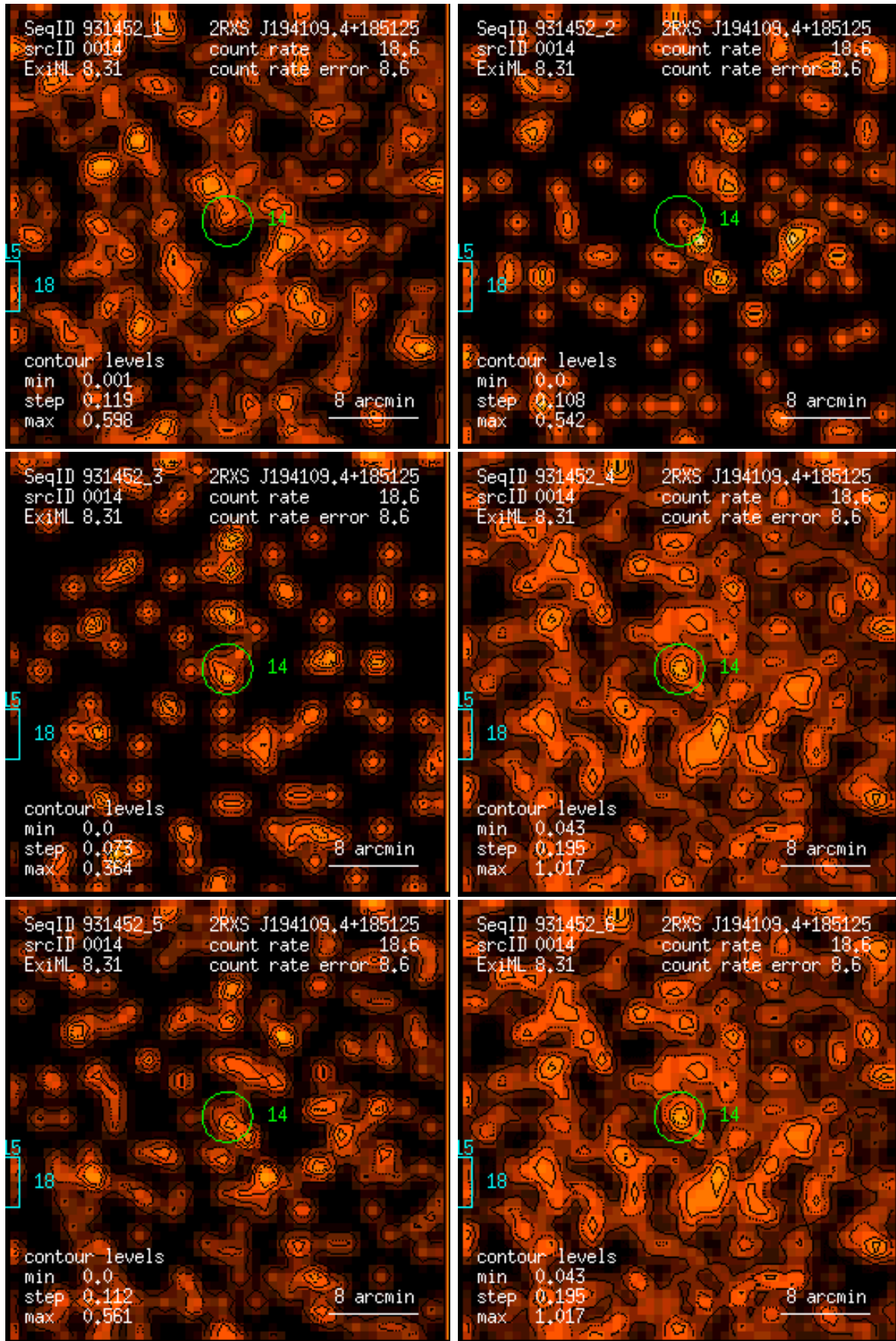
Figure 14: RASS 931452: detection 0014: band rate images, Gaussian filter: (1) PSPC channels 11 – 41, (2) 52 – 90, (3) 91 – 201, (4) 11 – 235, (5) 52 – 201, (6) 11 – 201. Broad band rates in counts/ks. Band rate contour levels in counts/ks/arcmin 2 .
