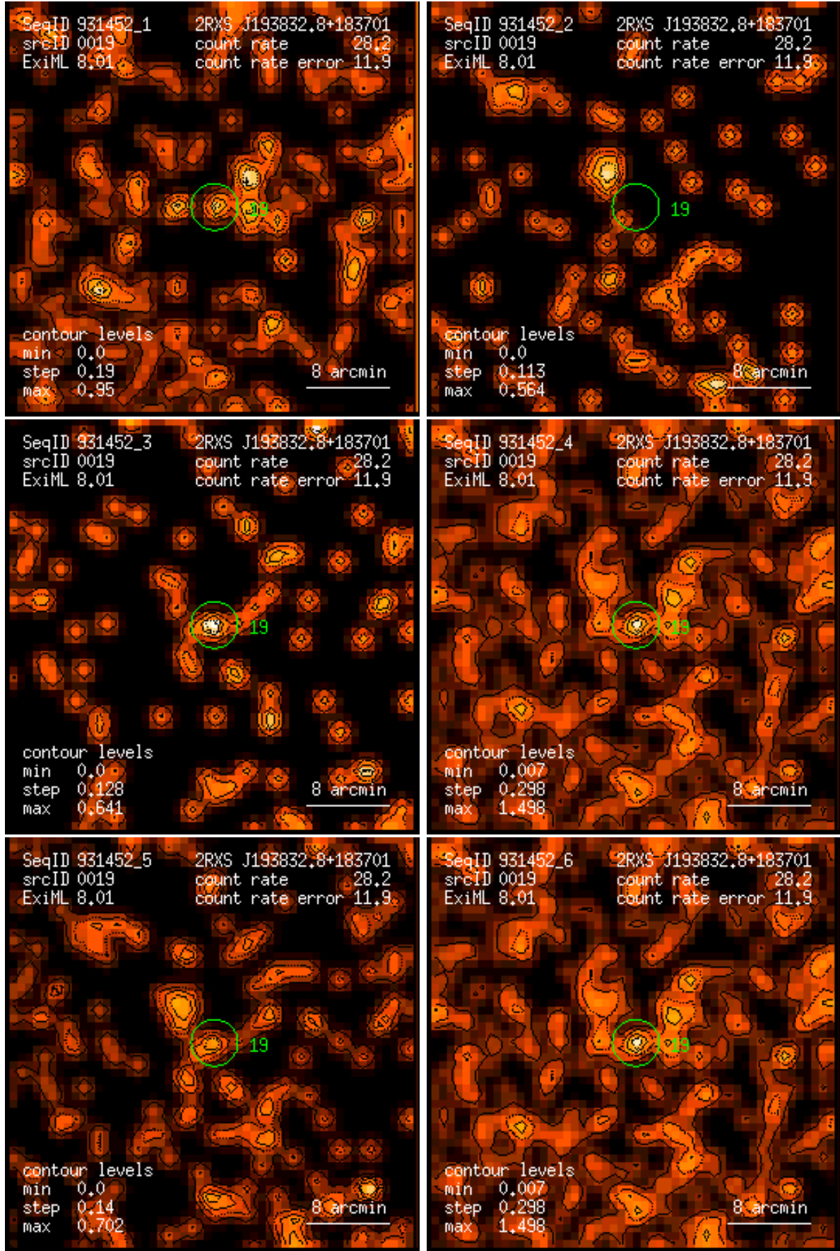
Figure 19: RASS 931452: detection 0019: band rate images, Gaussian filter: (1) PSPC channels 11 – 41, (2) 52 – 90, (3) 91 – 201, (4) 11 – 235, (5) 52 – 201, (6) 11 – 201. Broad band rates in counts/ks. Band rate contour levels in counts/ks/arcmin 2 .
