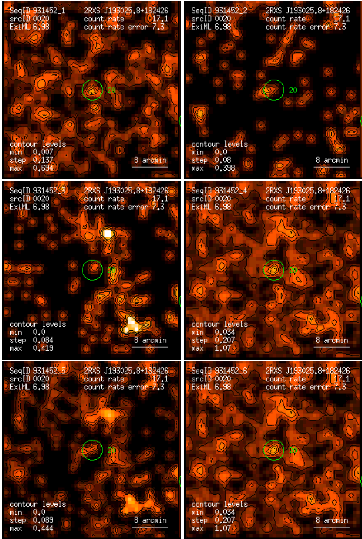
Figure 20: RASS 931452: detection 0020: band rate images, Gaussian filter: (1) PSPC channels 11 – 41, (2) 52 – 90, (3) 91 – 201, (4) 11 – 235, (5) 52 – 201, (6) 11 – 201. Broad band rates in counts/ks. Band rate contour levels in counts/ks/arcmin 2 .
