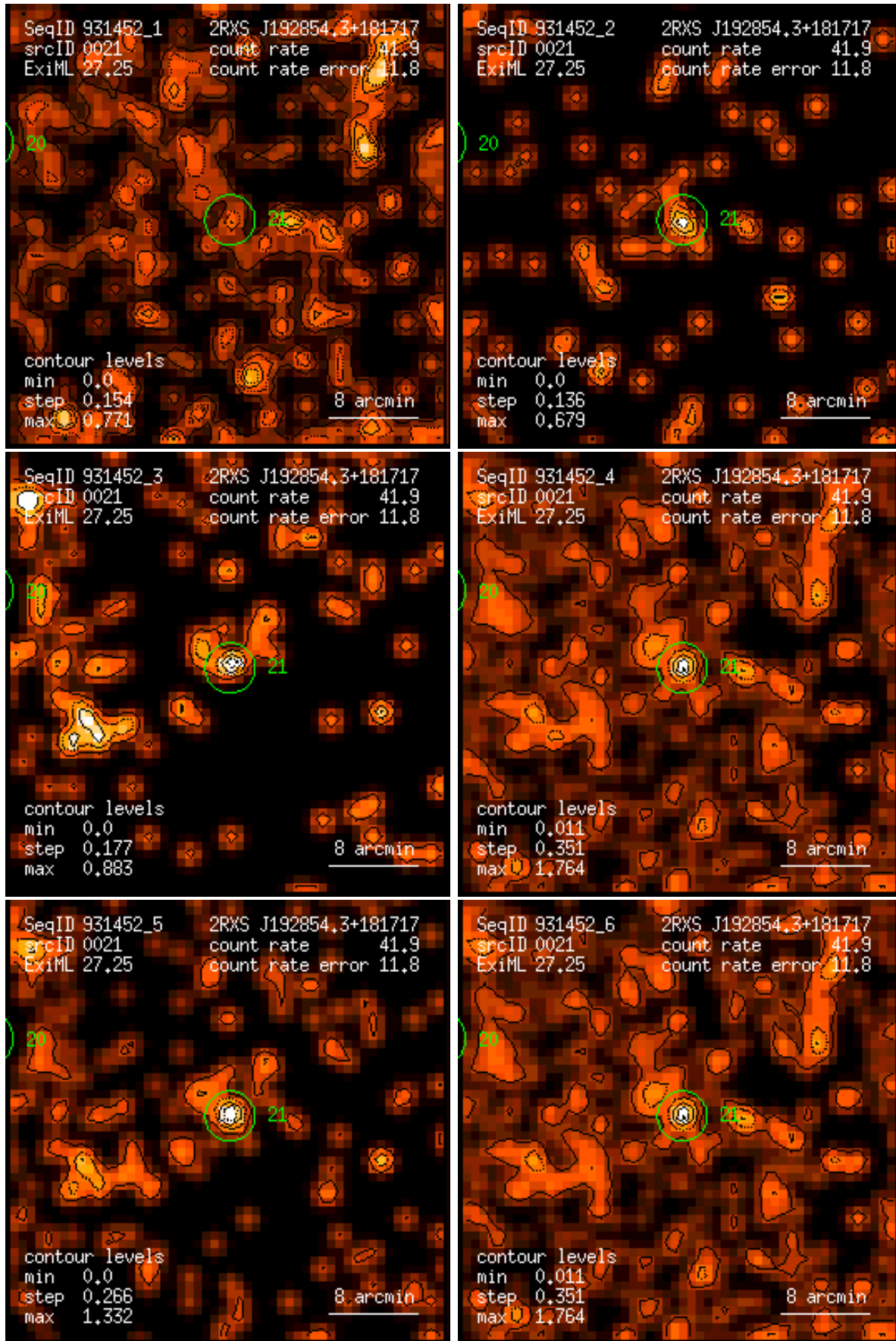
Figure 21: RASS 931452: detection 0021: band rate images, Gaussian filter: (1) PSPC channels 11 – 41, (2) 52 – 90, (3) 91 – 201, (4) 11 – 235, (5) 52 – 201, (6) 11 – 201. Broad band rates in counts/ks. Band rate contour levels in counts/ks/arcmin 2 .
