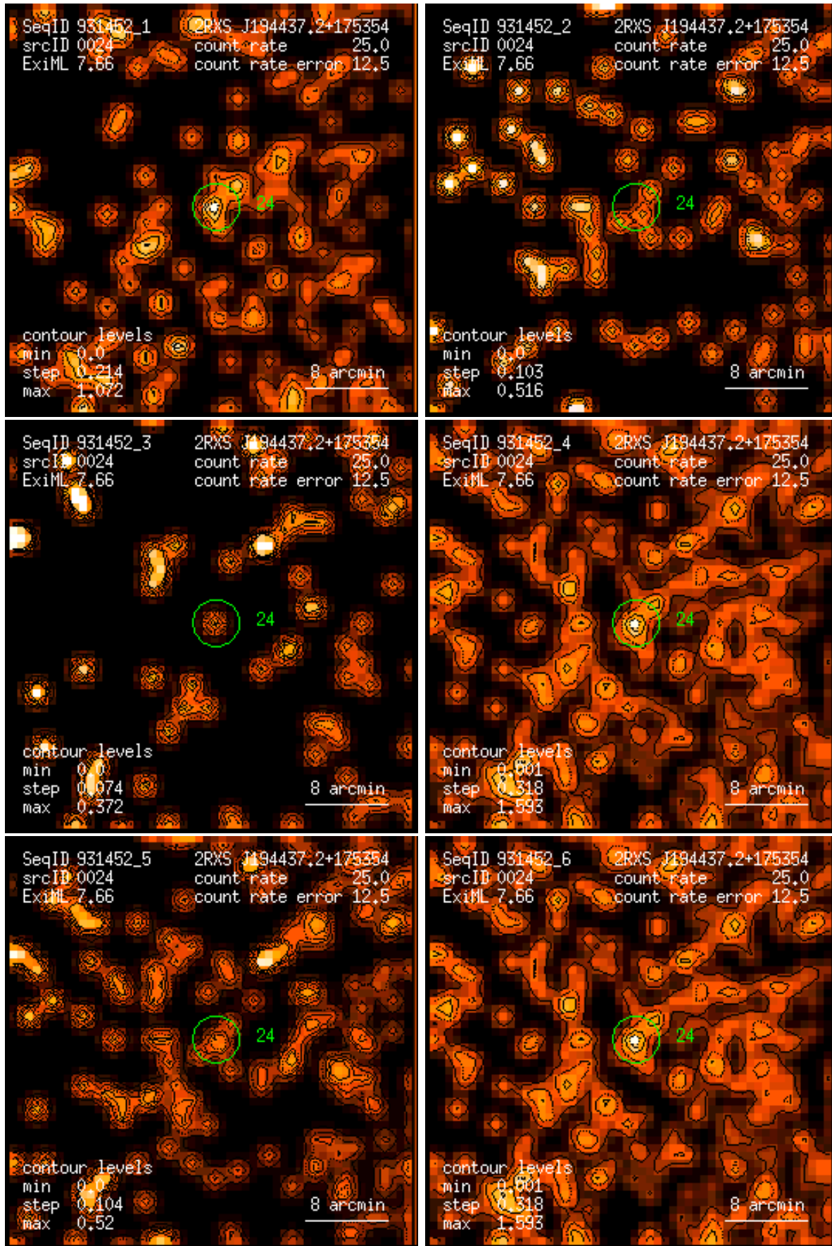
Figure 24: RASS 931452: detection 0024: band rate images, Gaussian filter: (1) PSPC channels 11 – 41, (2) 52 – 90, (3) 91 – 201, (4) 11 – 235, (5) 52 – 201, (6) 11 – 201. Broad band rates in counts/ks. Band rate contour levels in counts/ks/arcmin 2 .
