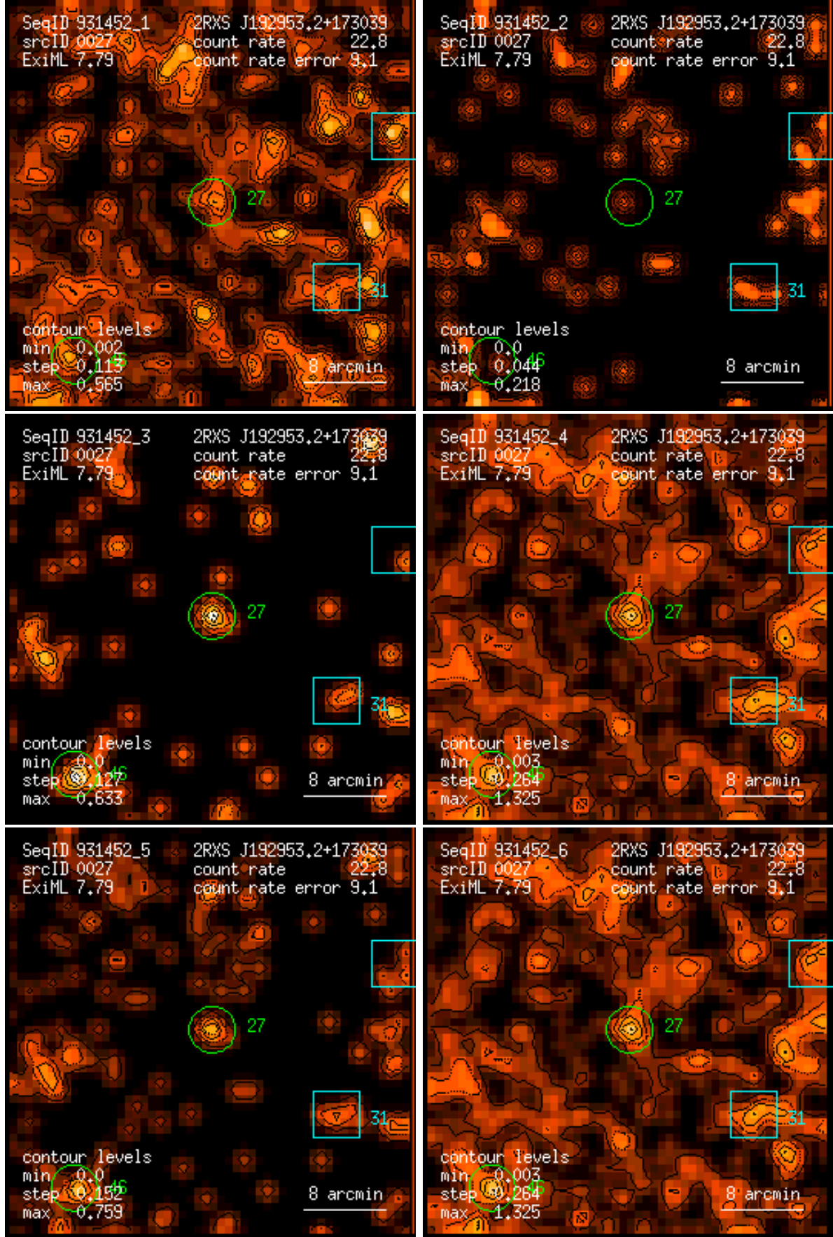
Figure 27: RASS 931452: detection 0027: band rate images, Gaussian filter: (1) PSPC channels 11 – 41, (2) 52 – 90, (3) 91 – 201, (4) 11 – 235, (5) 52 – 201, (6) 11 – 201. Broad band rates in counts/ks. Band rate contour levels in counts/ks/arcmin 2 .
