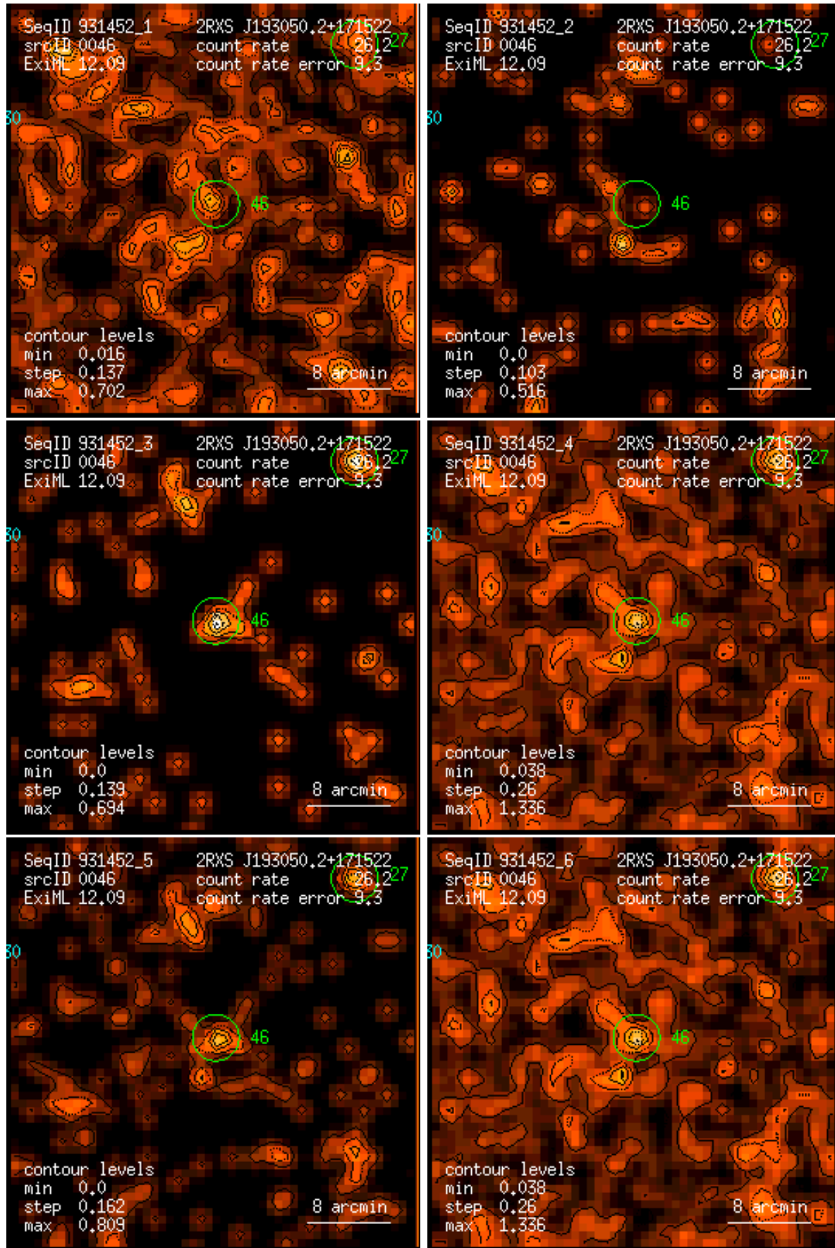
Figure 46: RASS 931452: detection 0046: band rate images, Gaussian filter: (1) PSPC channels 11 – 41, (2) 52 – 90, (3) 91 – 201, (4) 11 – 235, (5) 52 – 201, (6) 11 – 201. Broad band rates in counts/ks. Band rate contour levels in counts/ks/arcmin 2 .
