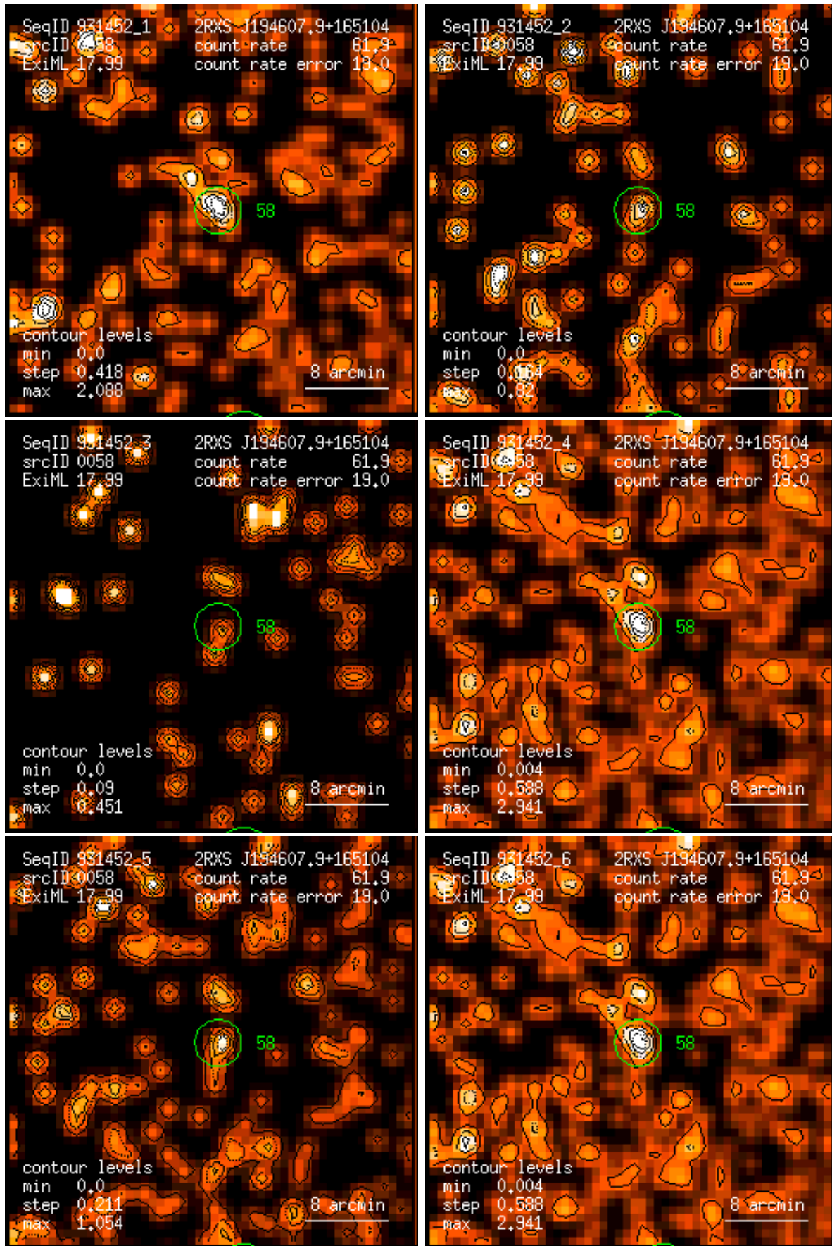
Figure 58: RASS 931452: detection 0058: band rate images, Gaussian filter: (1) PSPC channels 11 – 41, (2) 52 – 90, (3) 91 – 201, (4) 11 – 235, (5) 52 – 201, (6) 11 – 201. Broad band rates in counts/ks. Band rate contour levels in counts/ks/arcmin 2 .
