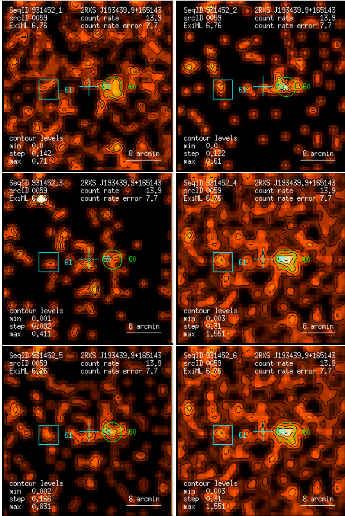
Figure 59: RASS 931452: detection 0059: band rate images, Gaussian filter: (1) PSPC channels 11 – 41, (2) 52 – 90, (3) 91 – 201, (4) 11 – 235, (5) 52 – 201, (6) 11 – 201. Broad band rates in counts/ks. Band rate contour levels in counts/ks/arcmin 2 .
