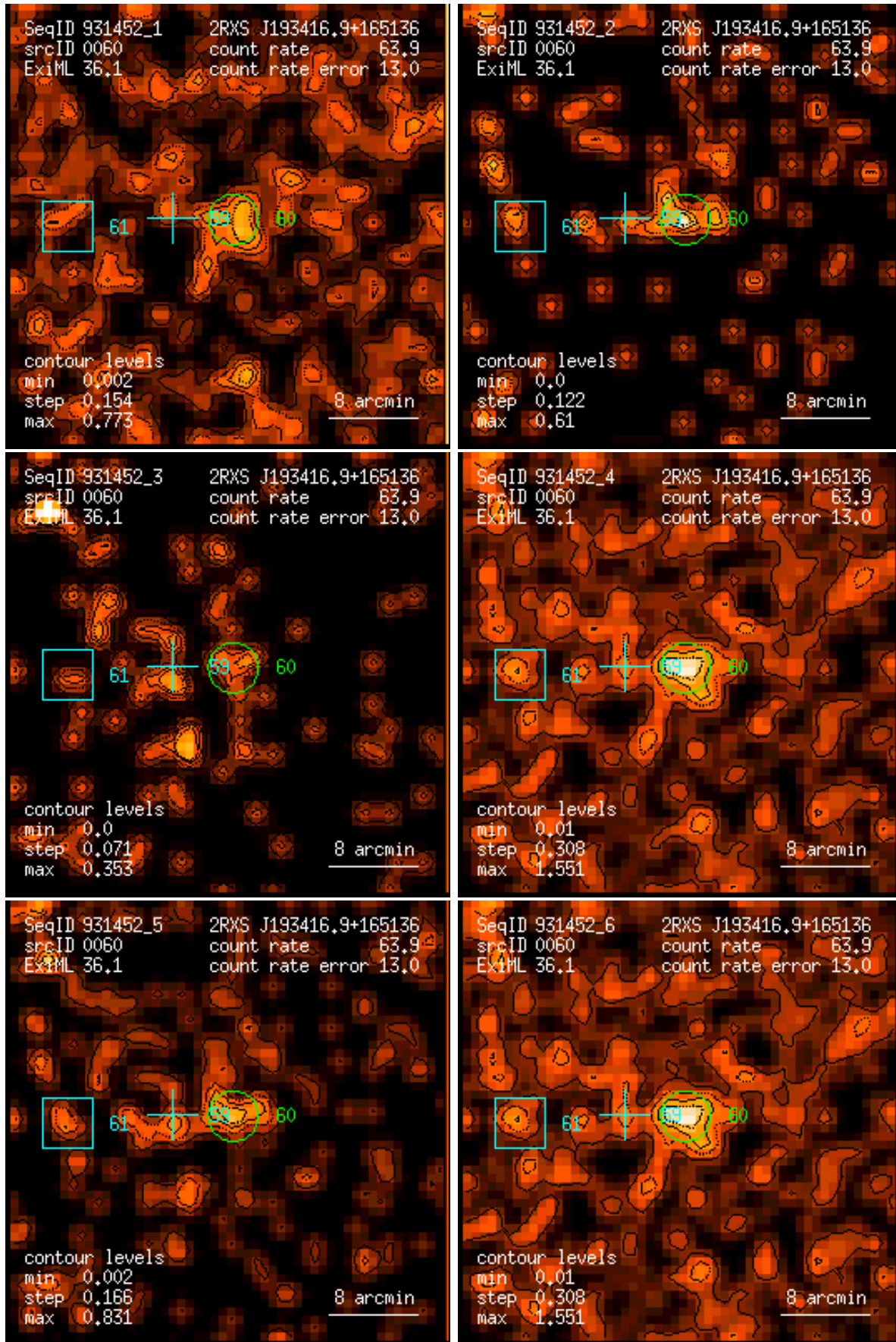
Figure 60: RASS 931452: detection 0060: band rate images, Gaussian filter: (1) PSPC channels 11 – 41, (2) 52 – 90, (3) 91 – 201, (4) 11 – 235, (5) 52 – 201, (6) 11 – 201. Broad band rates in counts/ks. Band rate contour levels in counts/ks/arcmin 2 .
