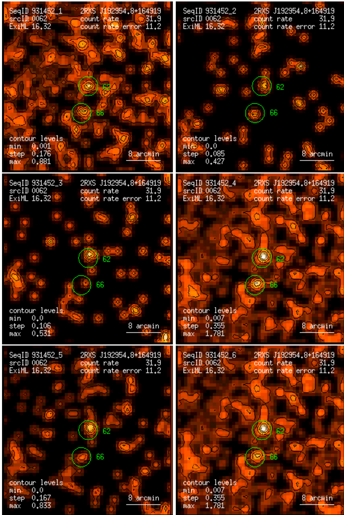
Figure 62: RASS 931452: detection 0062: band rate images, Gaussian filter: (1) PSPC channels 11 – 41, (2) 52 – 90, (3) 91 – 201, (4) 11 – 235, (5) 52 – 201, (6) 11 – 201. Broad band rates in counts/ks. Band rate contour levels in counts/ks/arcmin 2 .
