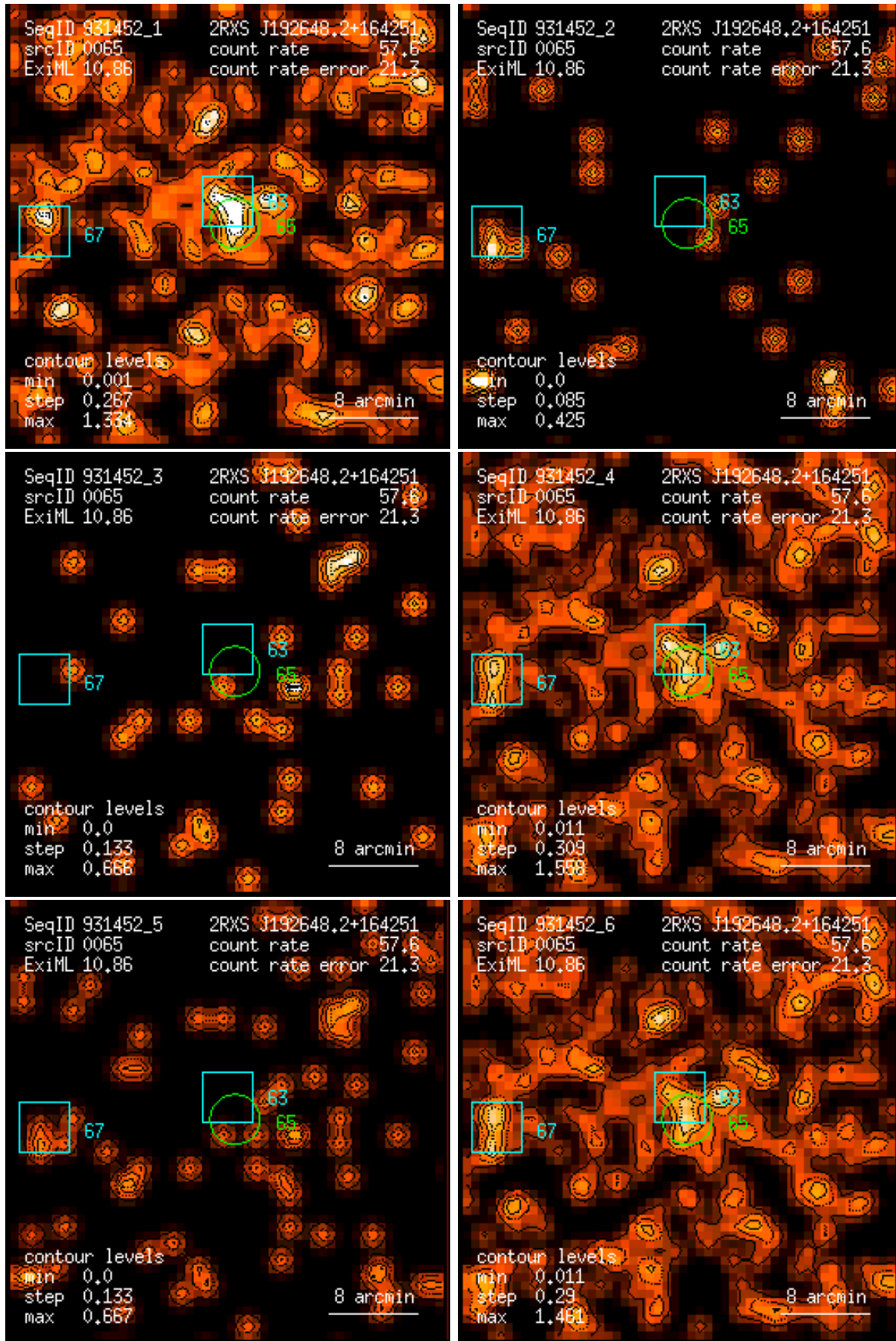
Figure 65: RASS 931452: detection 0065: band rate images, Gaussian filter: (1) PSPC channels 11 – 41, (2) 52 – 90, (3) 91 – 201, (4) 11 – 235, (5) 52 – 201, (6) 11 – 201. Broad band rates in counts/ks. Band rate contour levels in counts/ks/arcmin 2 .
