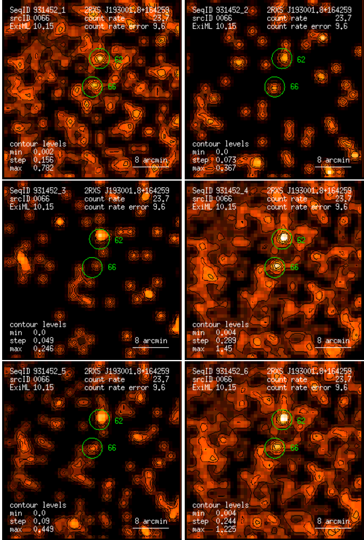
Figure 66: RASS 931452: detection 0066: band rate images, Gaussian filter: (1) PSPC channels 11 – 41, (2) 52 – 90, (3) 91 – 201, (4) 11 – 235, (5) 52 – 201, (6) 11 – 201. Broad band rates in counts/ks. Band rate contour levels in counts/ks/arcmin 2 .
