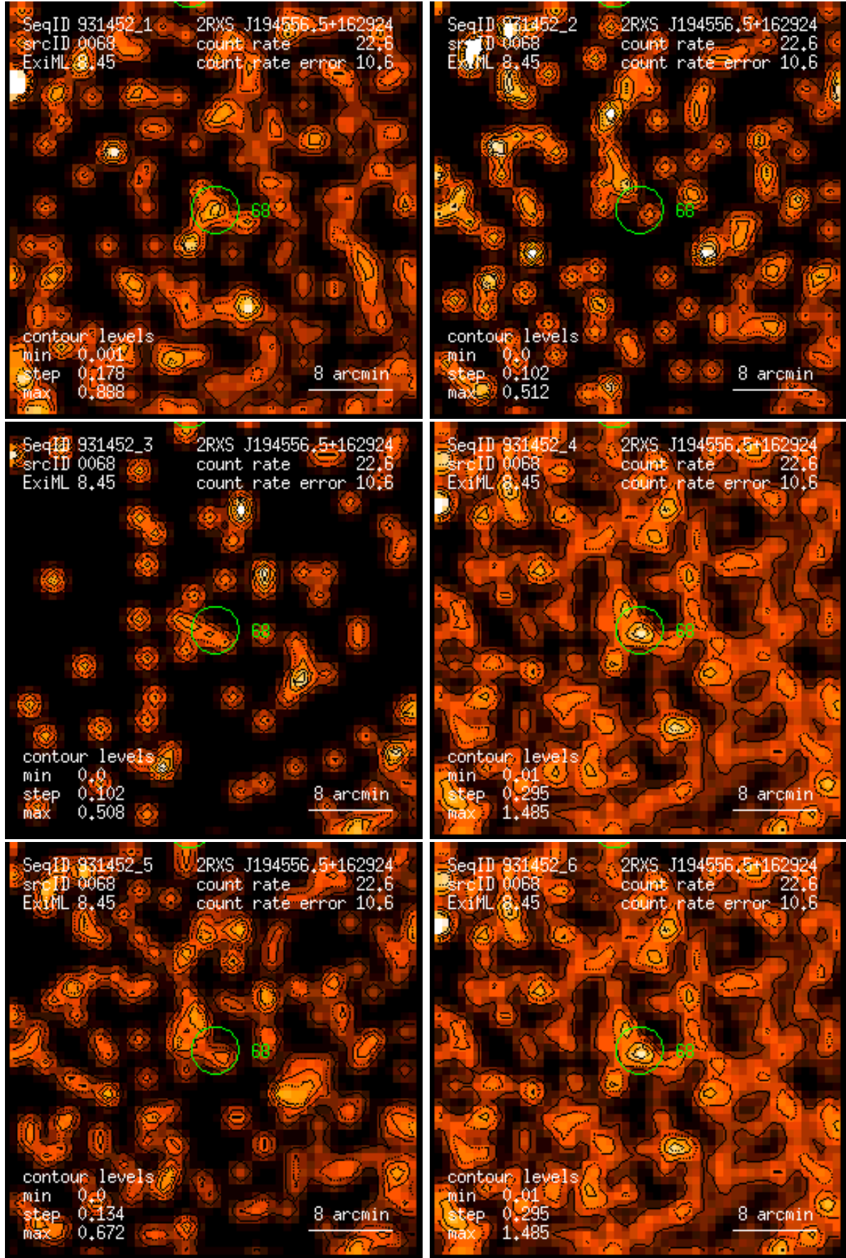
Figure 68: RASS 931452: detection 0068: band rate images, Gaussian filter: (1) PSPC channels 11 – 41, (2) 52 – 90, (3) 91 – 201, (4) 11 – 235, (5) 52 – 201, (6) 11 – 201. Broad band rates in counts/ks. Band rate contour levels in counts/ks/arcmin 2 .
