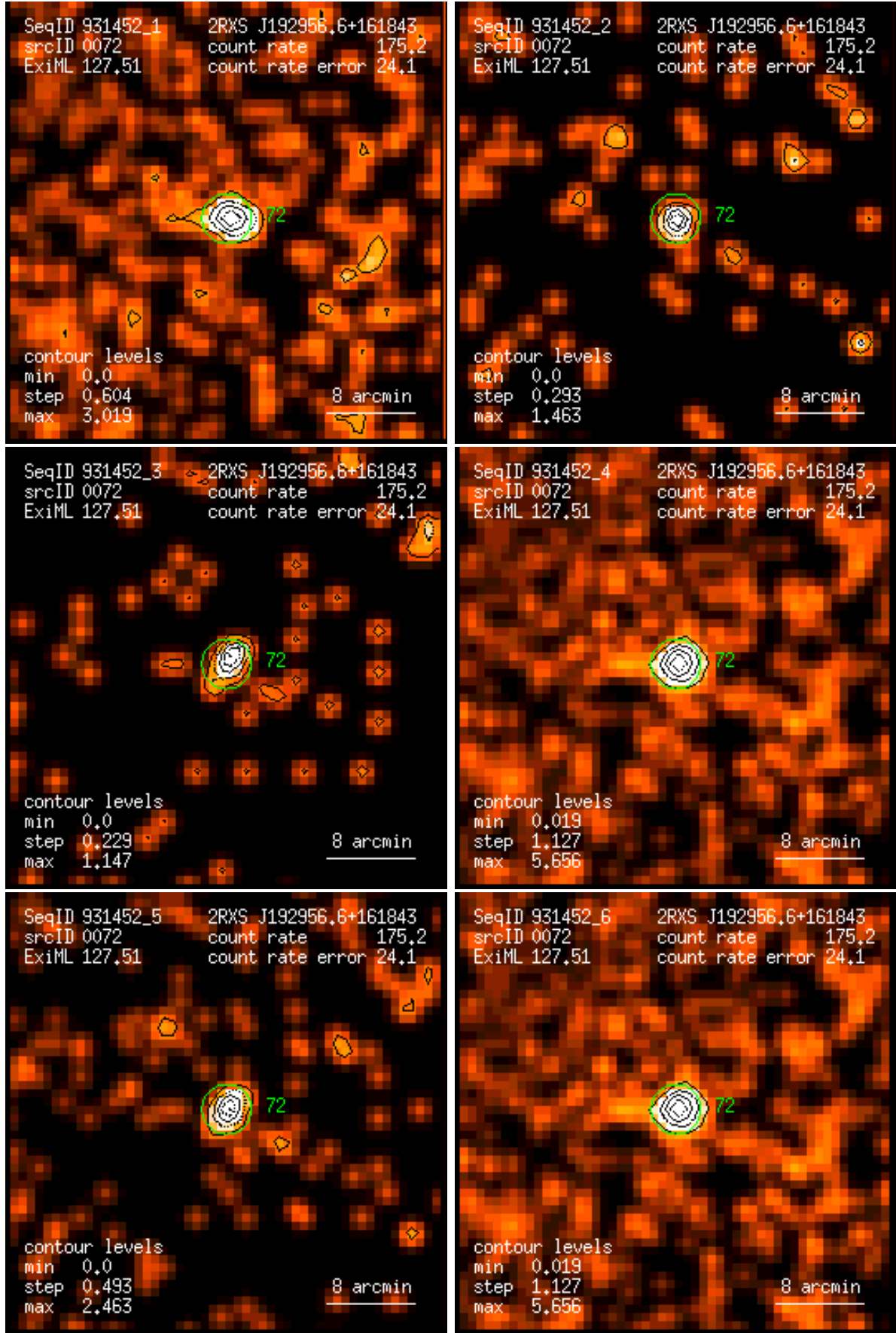
Figure 72: RASS 931452: detection 0072: band rate images, Gaussian filter: (1) PSPC channels 11 – 41, (2) 52 – 90, (3) 91 – 201, (4) 11 – 235, (5) 52 – 201, (6) 11 – 201. Broad band rates in counts/ks. Band rate contour levels in counts/ks/arcmin 2 .
