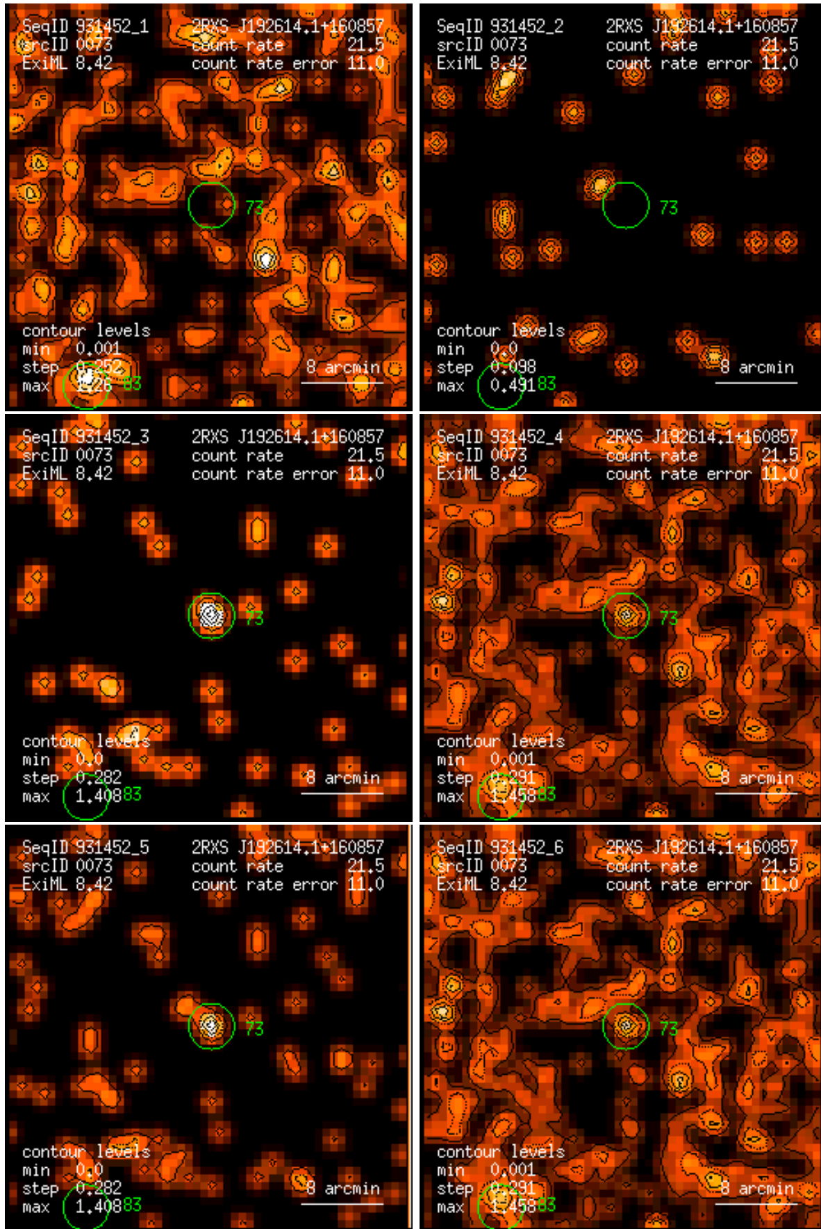
Figure 73: RASS 931452: detection 0073: band rate images, Gaussian filter: (1) PSPC channels 11 – 41, (2) 52 – 90, (3) 91 – 201, (4) 11 – 235, (5) 52 – 201, (6) 11 – 201. Broad band rates in counts/ks. Band rate contour levels in counts/ks/arcmin 2 .
