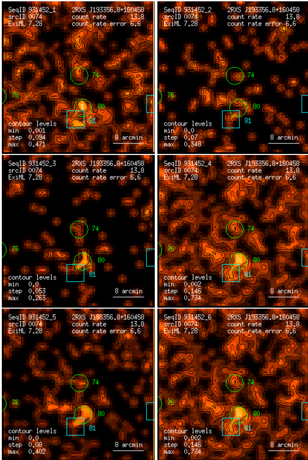
Figure 74: RASS 931452: detection 0074: band rate images, Gaussian filter: (1) PSPC channels 11 – 41, (2) 52 – 90, (3) 91 – 201, (4) 11 – 235, (5) 52 – 201, (6) 11 – 201. Broad band rates in counts/ks. Band rate contour levels in counts/ks/arcmin 2 .
