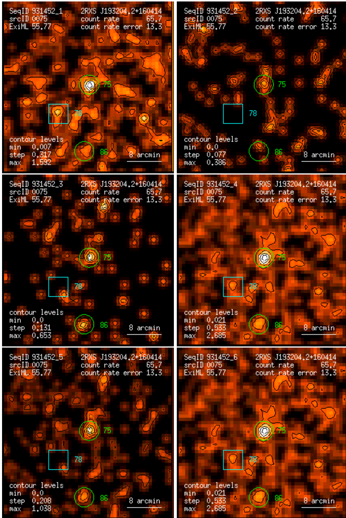
Figure 75: RASS 931452: detection 0075: band rate images, Gaussian filter: (1) PSPC channels 11 – 41, (2) 52 – 90, (3) 91 – 201, (4) 11 – 235, (5) 52 – 201, (6) 11 – 201. Broad band rates in counts/ks. Band rate contour levels in counts/ks/arcmin 2 .
