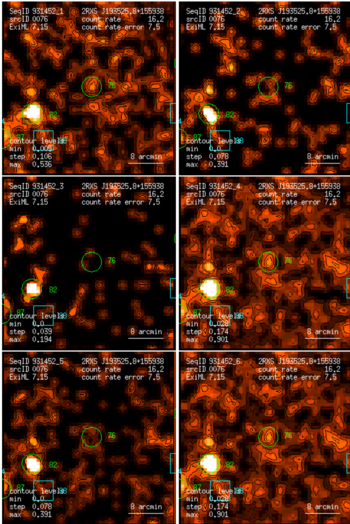
Figure 76: RASS 931452: detection 0076: band rate images, Gaussian filter: (1) PSPC channels 11 – 41, (2) 52 – 90, (3) 91 – 201, (4) 11 – 235, (5) 52 – 201, (6) 11 – 201. Broad band rates in counts/ks. Band rate contour levels in counts/ks/arcmin 2 .
