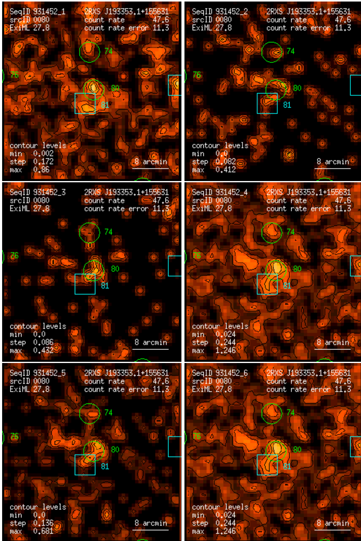
Figure 80: RASS 931452: detection 0080: band rate images, Gaussian filter: (1) PSPC channels 11 – 41, (2) 52 – 90, (3) 91 – 201, (4) 11 – 235, (5) 52 – 201, (6) 11 – 201. Broad band rates in counts/ks. Band rate contour levels in counts/ks/arcmin 2 .
