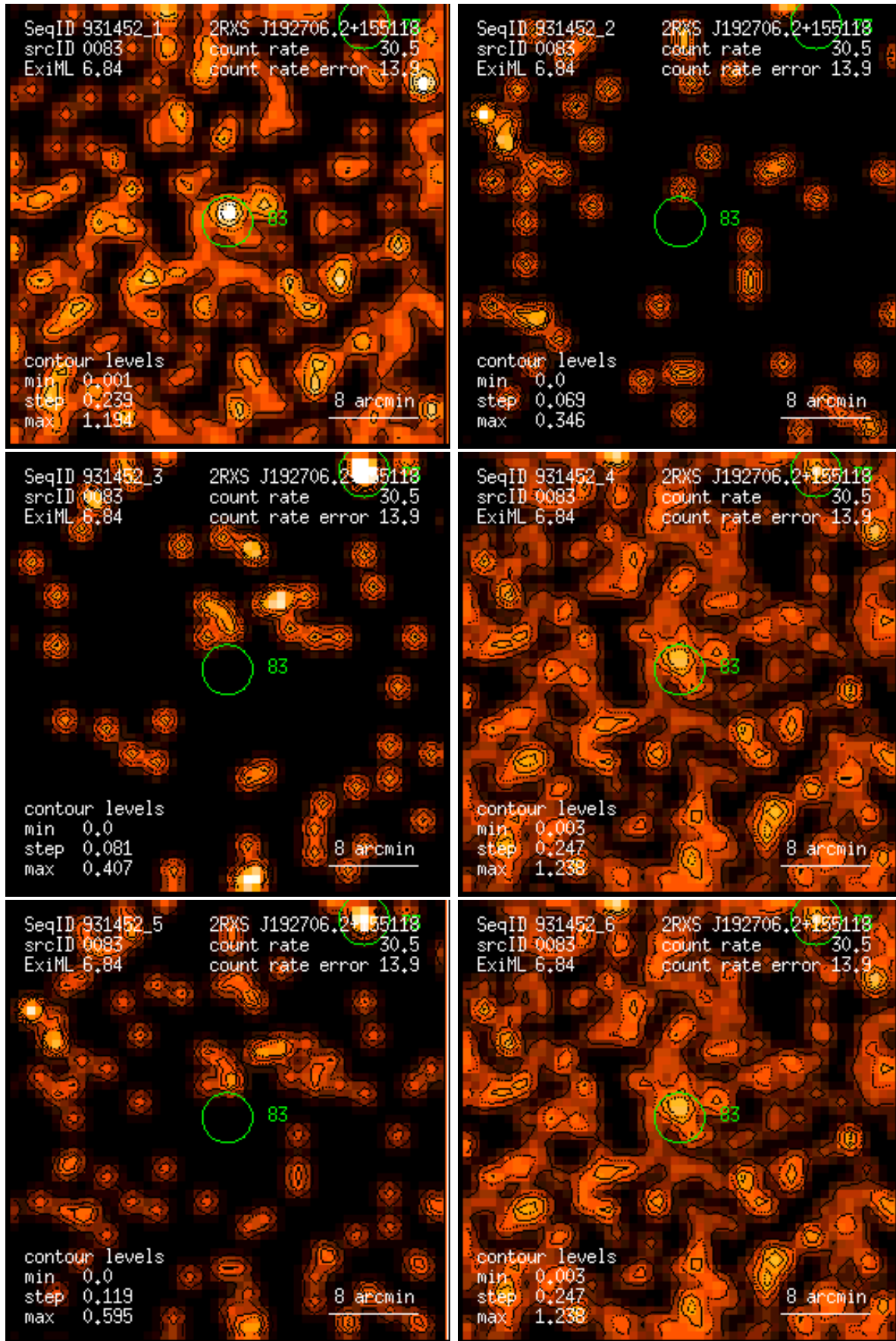
Figure 83: RASS 931452: detection 0083: band rate images, Gaussian filter: (1) PSPC channels 11 – 41, (2) 52 – 90, (3) 91 – 201, (4) 11 – 235, (5) 52 – 201, (6) 11 – 201. Broad band rates in counts/ks. Band rate contour levels in counts/ks/arcmin 2 .
