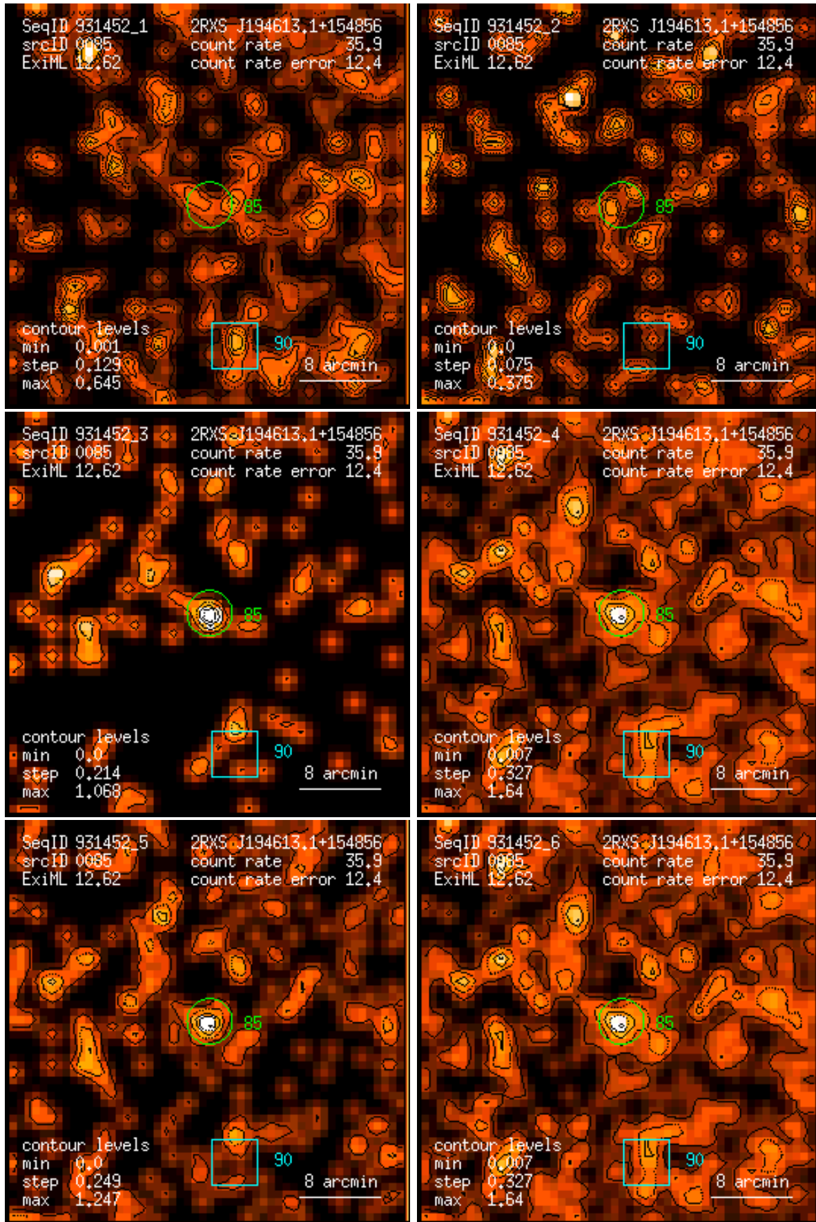
Figure 85: RASS 931452: detection 0085: band rate images, Gaussian filter: (1) PSPC channels 11 – 41, (2) 52 – 90, (3) 91 – 201, (4) 11 – 235, (5) 52 – 201, (6) 11 – 201. Broad band rates in counts/ks. Band rate contour levels in counts/ks/arcmin 2 .
