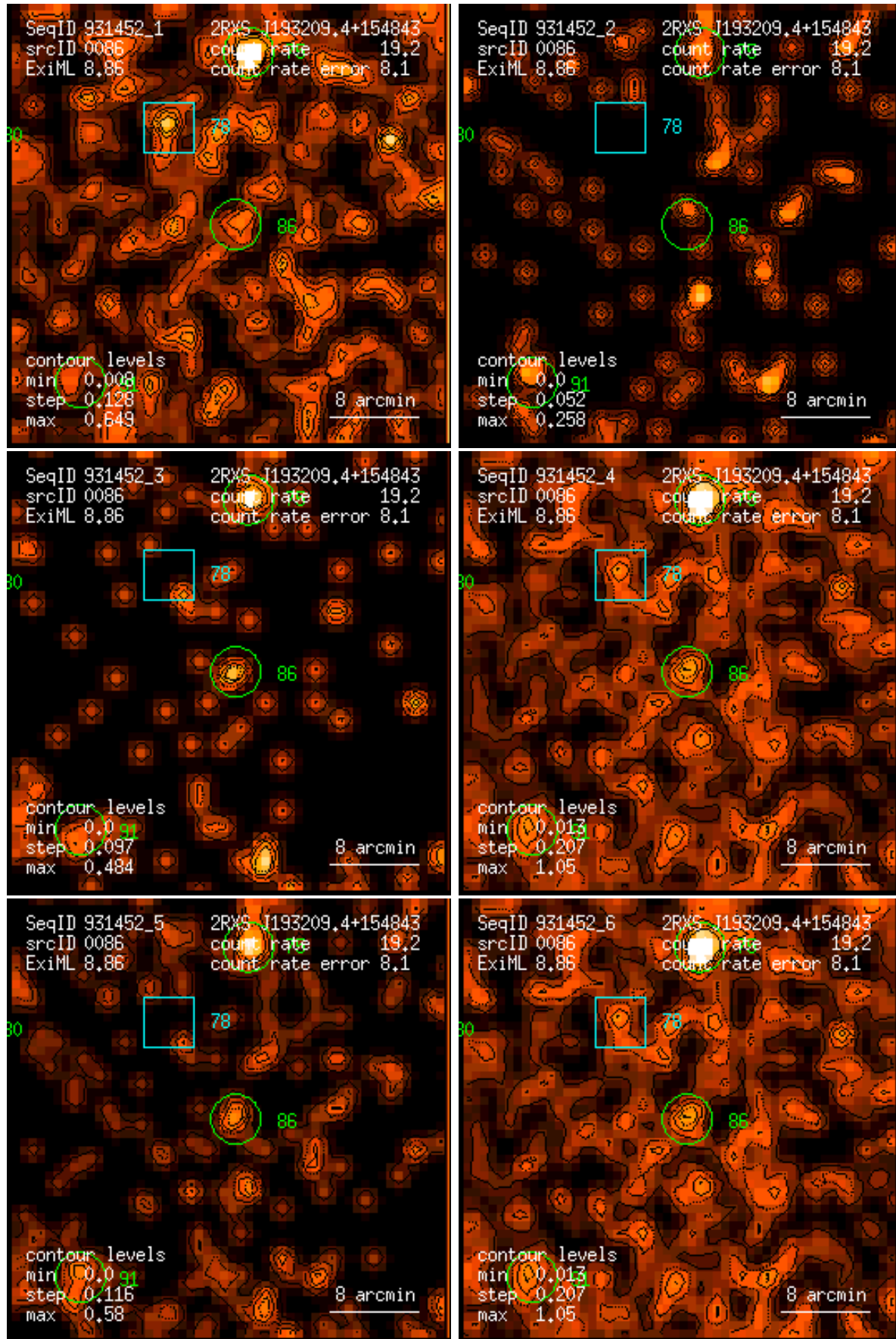
Figure 86: RASS 931452: detection 0086: band rate images, Gaussian filter: (1) PSPC channels 11 – 41, (2) 52 – 90, (3) 91 – 201, (4) 11 – 235, (5) 52 – 201, (6) 11 – 201. Broad band rates in counts/ks. Band rate contour levels in counts/ks/arcmin 2 .
