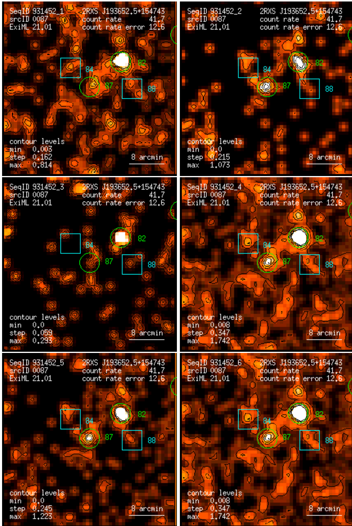
Figure 87: RASS 931452: detection 0087: band rate images, Gaussian filter: (1) PSPC channels 11 – 41, (2) 52 – 90, (3) 91 – 201, (4) 11 – 235, (5) 52 – 201, (6) 11 – 201. Broad band rates in counts/ks. Band rate contour levels in counts/ks/arcmin 2 .
