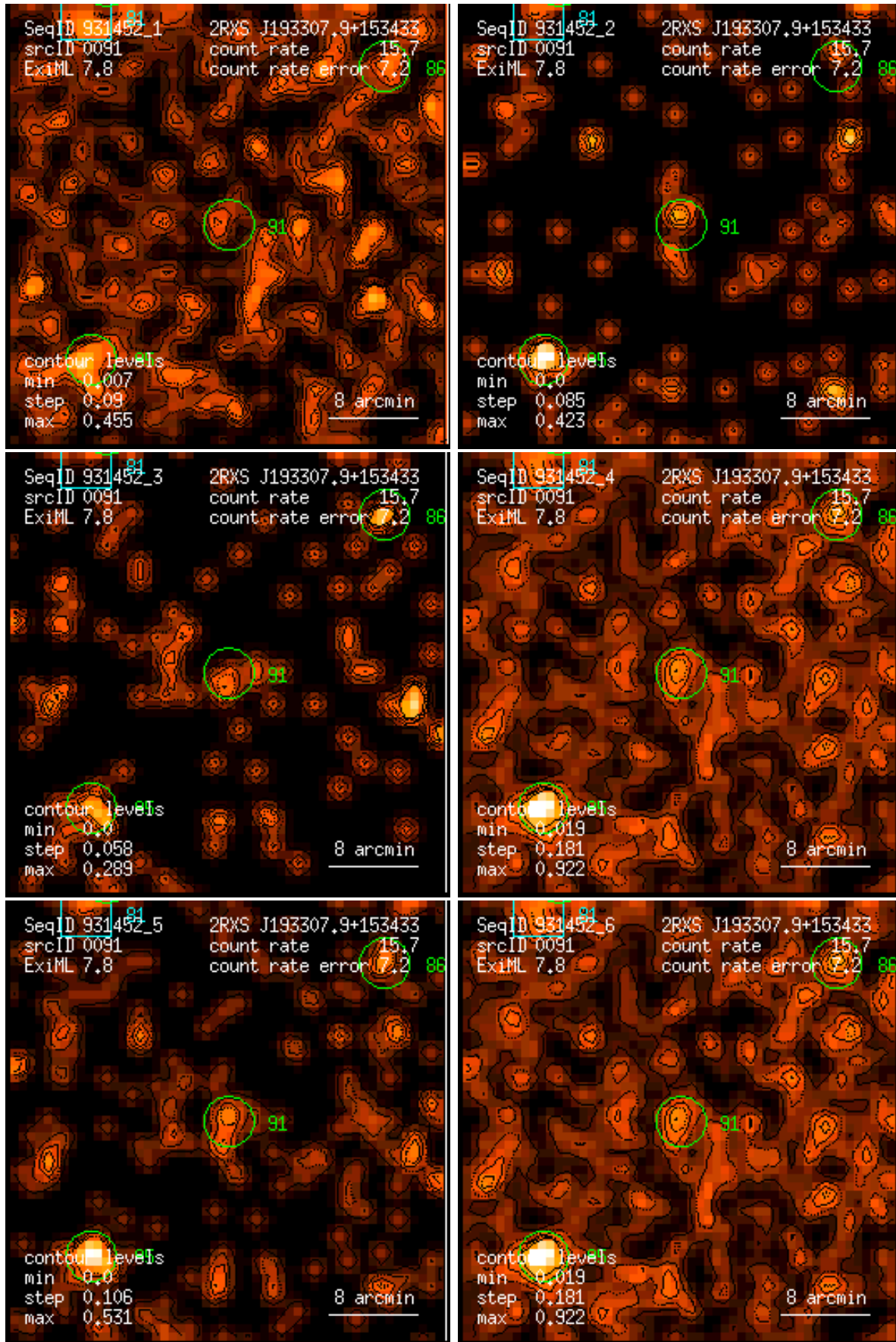
Figure 91: RASS 931452: detection 0091: band rate images, Gaussian filter: (1) PSPC channels 11 – 41, (2) 52 – 90, (3) 91 – 201, (4) 11 – 235, (5) 52 – 201, (6) 11 – 201. Broad band rates in counts/ks. Band rate contour levels in counts/ks/arcmin 2 .
