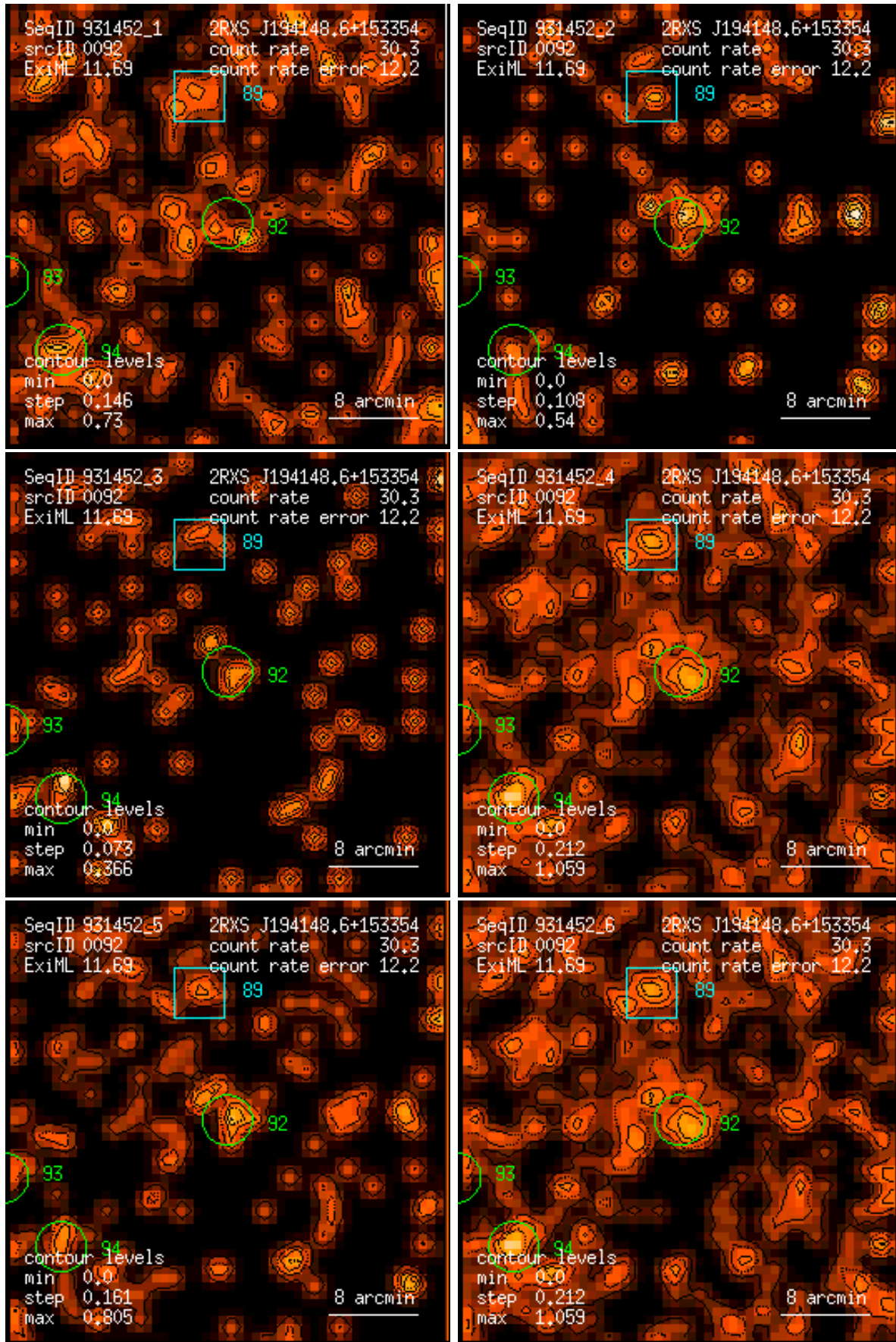
Figure 92: RASS 931452: detection 0092: band rate images, Gaussian filter: (1) PSPC channels 11 – 41, (2) 52 – 90, (3) 91 – 201, (4) 11 – 235, (5) 52 – 201, (6) 11 – 201. Broad band rates in counts/ks. Band rate contour levels in counts/ks/arcmin 2 .
