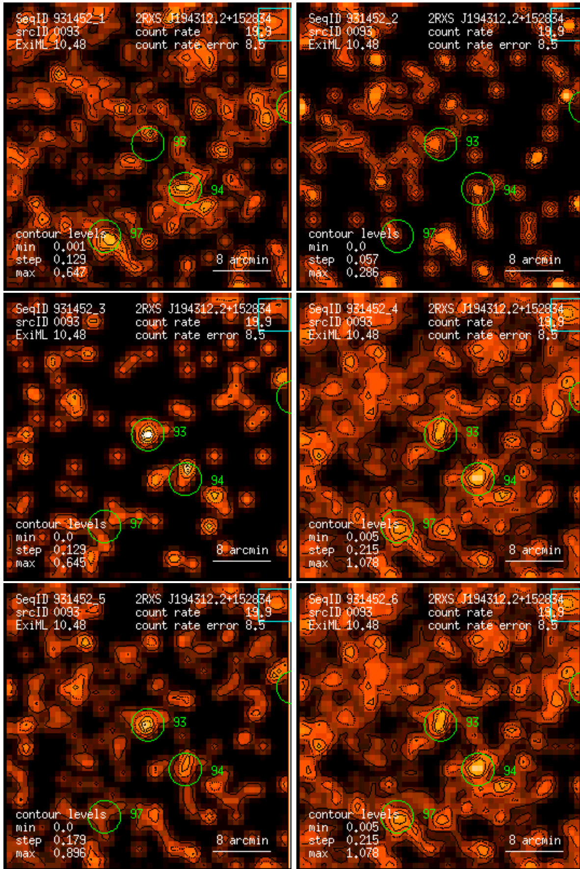
Figure 93: RASS 931452: detection 0093: band rate images, Gaussian filter: (1) PSPC channels 11 – 41, (2) 52 – 90, (3) 91 – 201, (4) 11 – 235, (5) 52 – 201, (6) 11 – 201. Broad band rates in counts/ks. Band rate contour levels in counts/ks/arcmin 2 .
