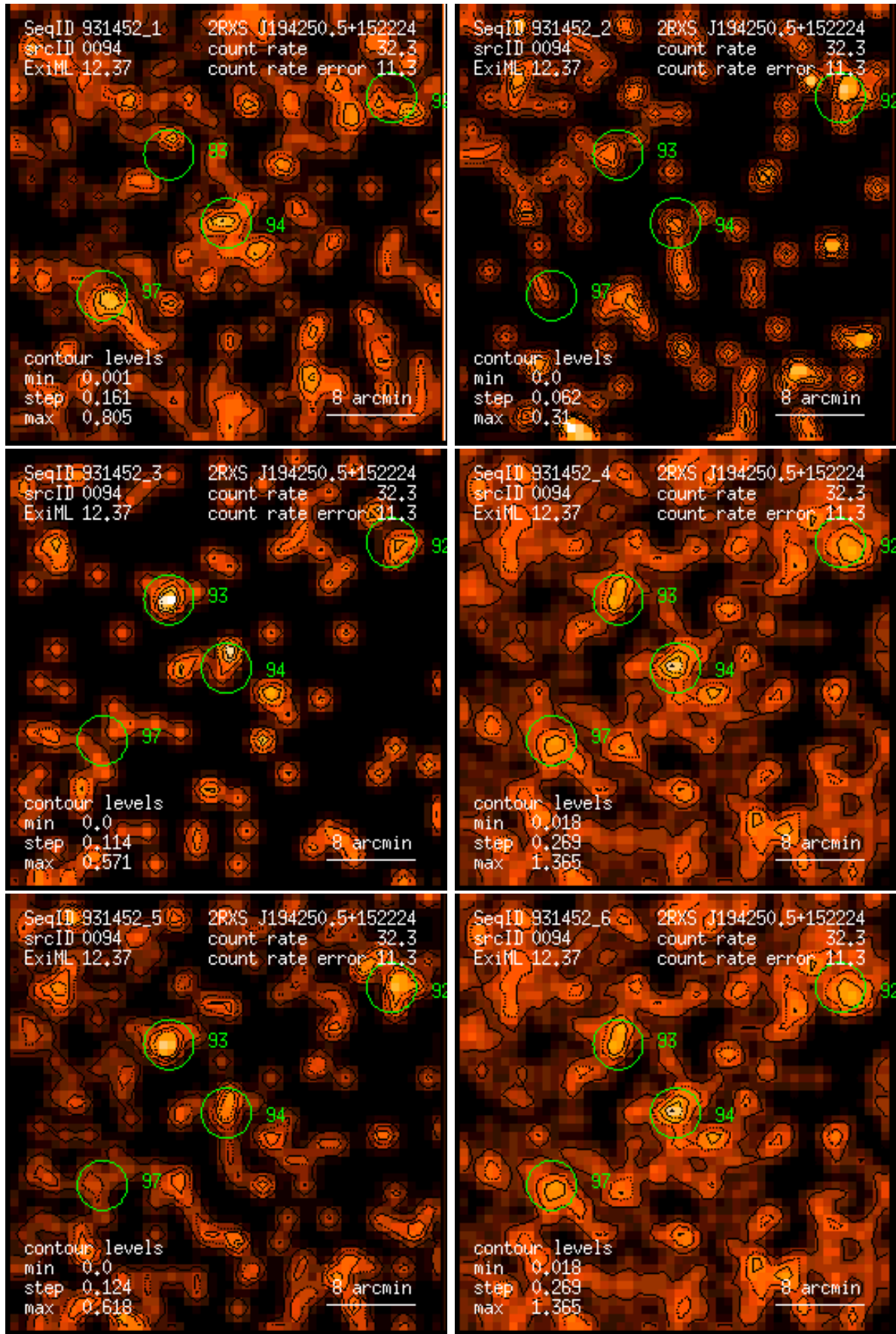
Figure 94: RASS 931452: detection 0094: band rate images, Gaussian filter: (1) PSPC channels 11 – 41, (2) 52 – 90, (3) 91 – 201, (4) 11 – 235, (5) 52 – 201, (6) 11 – 201. Broad band rates in counts/ks. Band rate contour levels in counts/ks/arcmin 2 .
