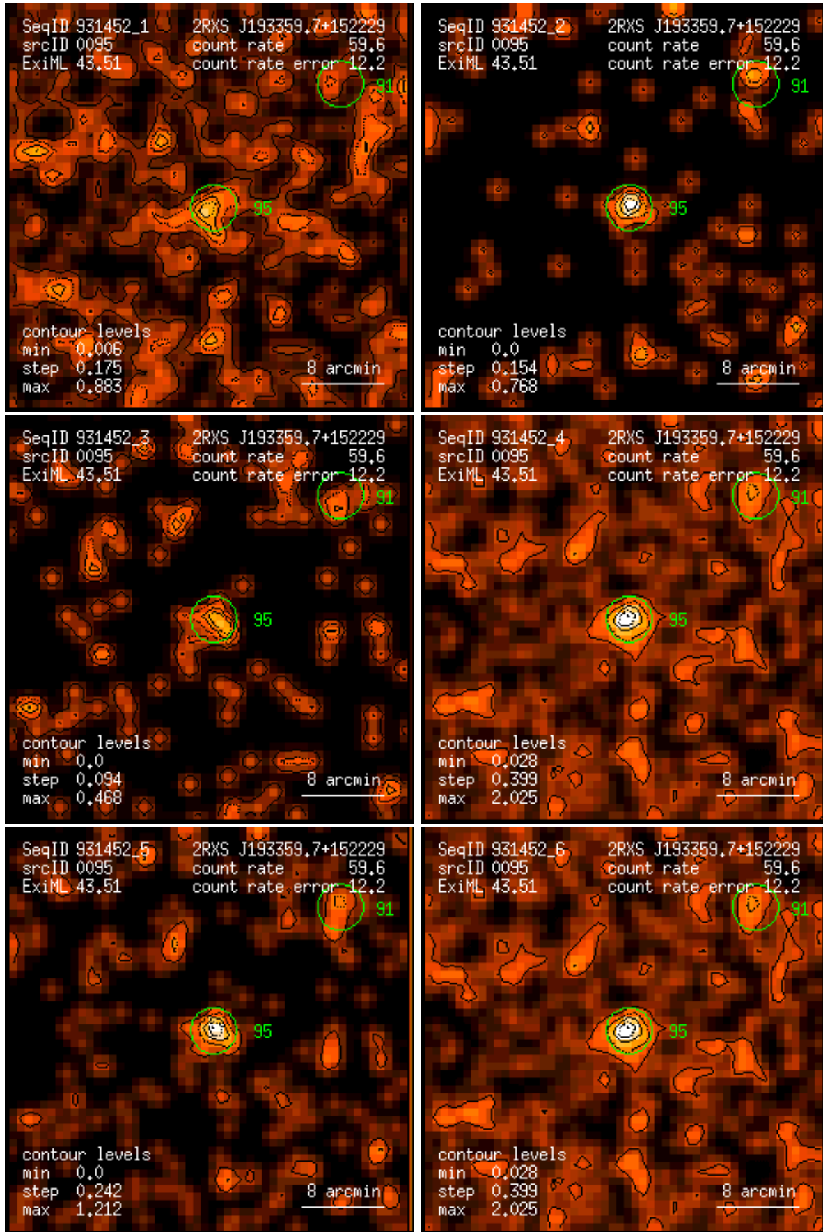
Figure 95: RASS 931452: detection 0095: band rate images, Gaussian filter: (1) PSPC channels 11 – 41, (2) 52 – 90, (3) 91 – 201, (4) 11 – 235, (5) 52 – 201, (6) 11 – 201. Broad band rates in counts/ks. Band rate contour levels in counts/ks/arcmin 2 .
