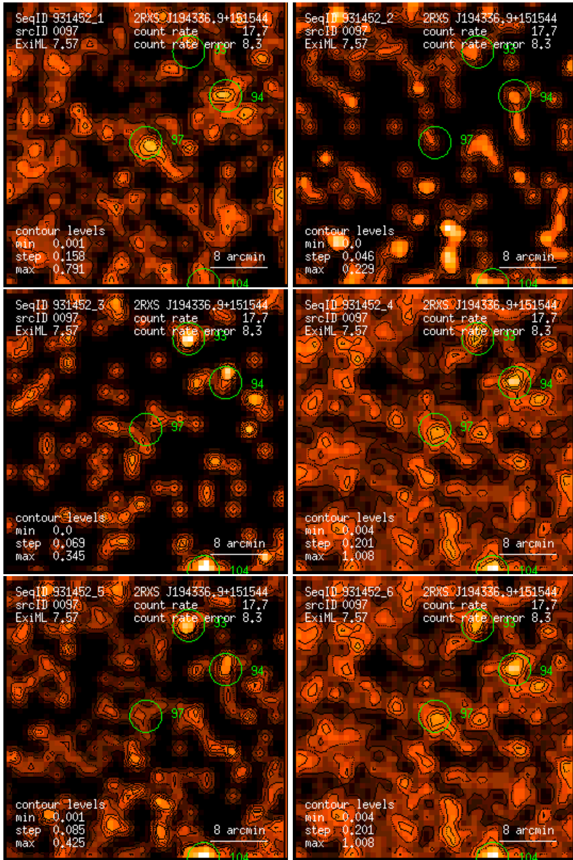
Figure 97: RASS 931452: detection 0097: band rate images, Gaussian filter: (1) PSPC channels 11 – 41, (2) 52 – 90, (3) 91 – 201, (4) 11 – 235, (5) 52 – 201, (6) 11 – 201. Broad band rates in counts/ks. Band rate contour levels in counts/ks/arcmin 2 .
