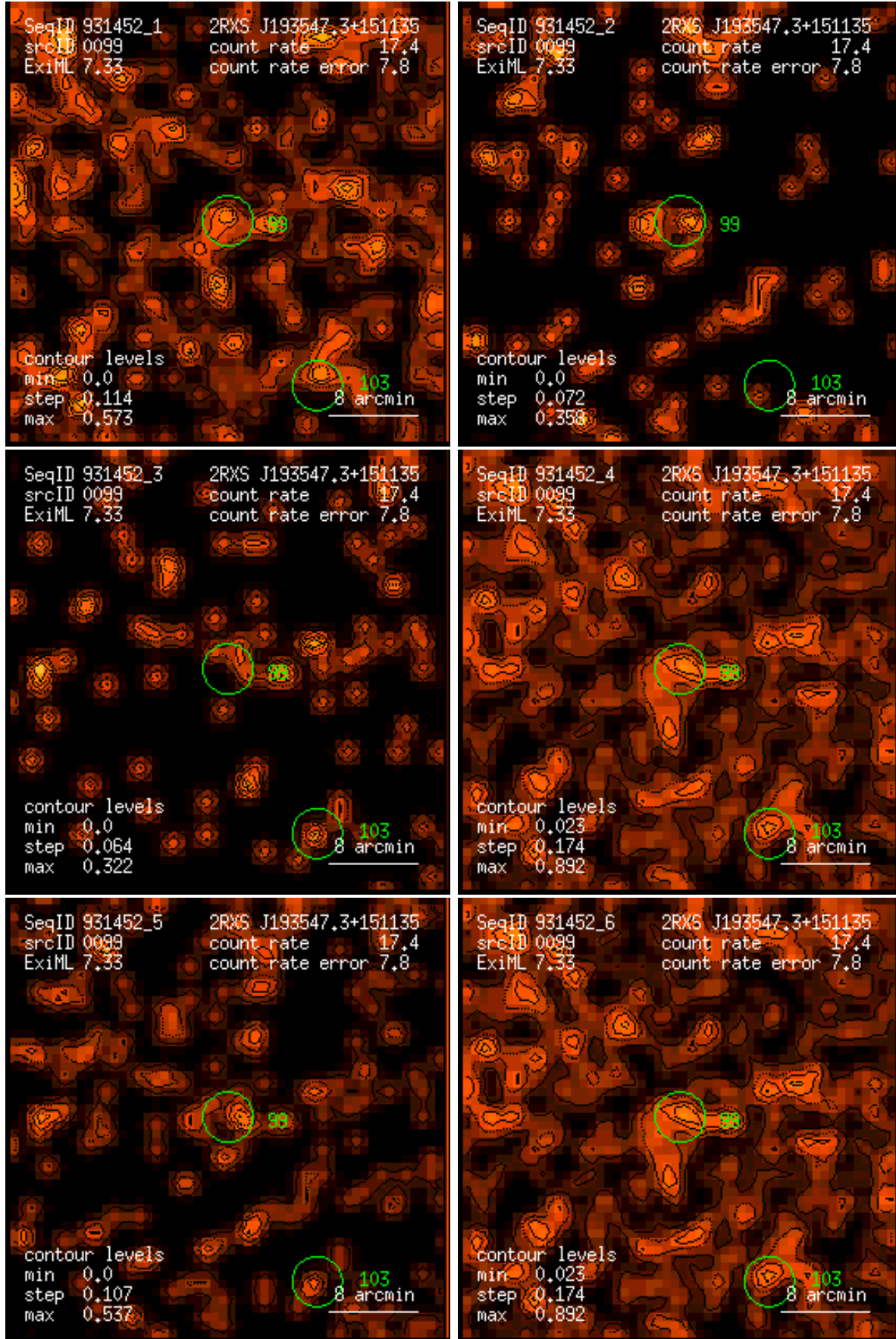
Figure 99: RASS 931452: detection 0099: band rate images, Gaussian filter: (1) PSPC channels 11 – 41, (2) 52 – 90, (3) 91 – 201, (4) 11 – 235, (5) 52 – 201, (6) 11 – 201. Broad band rates in counts/ks. Band rate contour levels in counts/ks/arcmin 2 .
