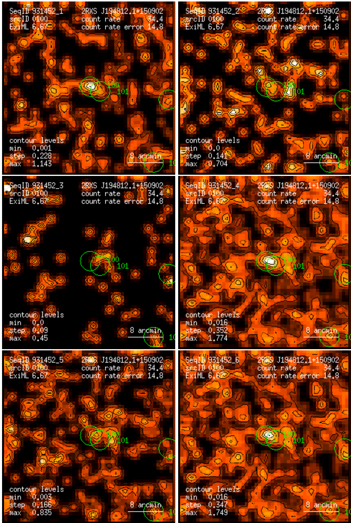
Figure 100: RASS 931452: detection 0100: band rate images, Gaussian filter: (1) PSPC channels 11 – 41, (2) 52 – 90, (3) 91 – 201, (4) 11 – 235, (5) 52 – 201, (6) 11 – 201. Broad band rates in counts/ks. Band rate contour levels in counts/ks/arcmin 2 .
