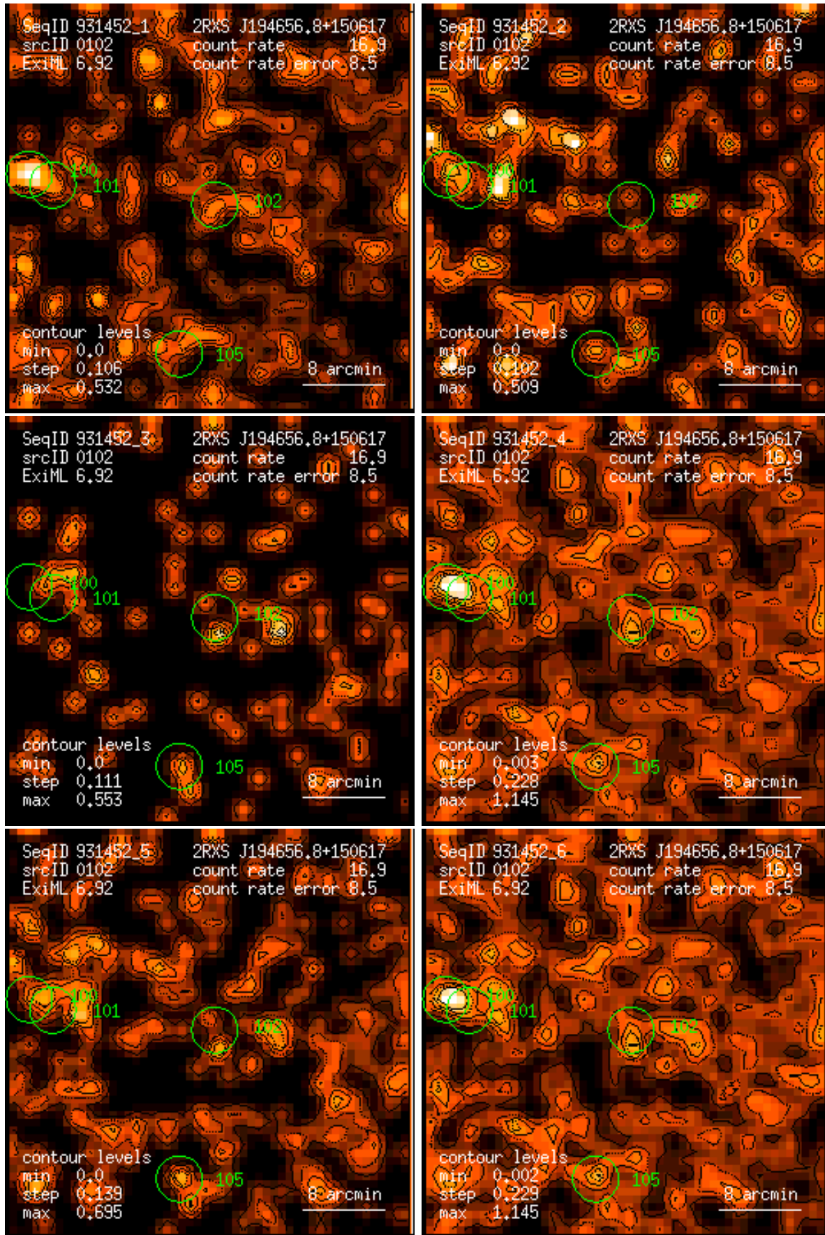
Figure 102: RASS 931452: detection 0102: band rate images, Gaussian filter: (1) PSPC channels 11 – 41, (2) 52 – 90, (3) 91 – 201, (4) 11 – 235, (5) 52 – 201, (6) 11 – 201. Broad band rates in counts/ks. Band rate contour levels in counts/ks/arcmin 2 .
