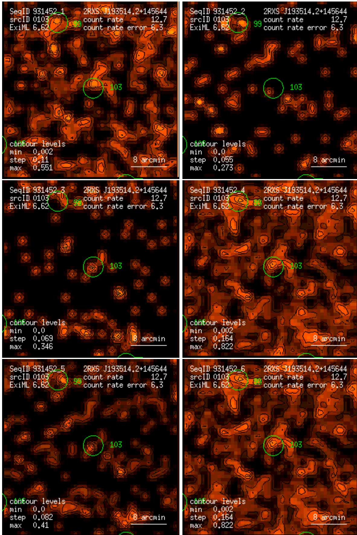
Figure 103: RASS 931452: detection 0103: band rate images, Gaussian filter: (1) PSPC channels 11 – 41, (2) 52 – 90, (3) 91 – 201, (4) 11 – 235, (5) 52 – 201, (6) 11 – 201. Broad band rates in counts/ks. Band rate contour levels in counts/ks/arcmin 2 .
