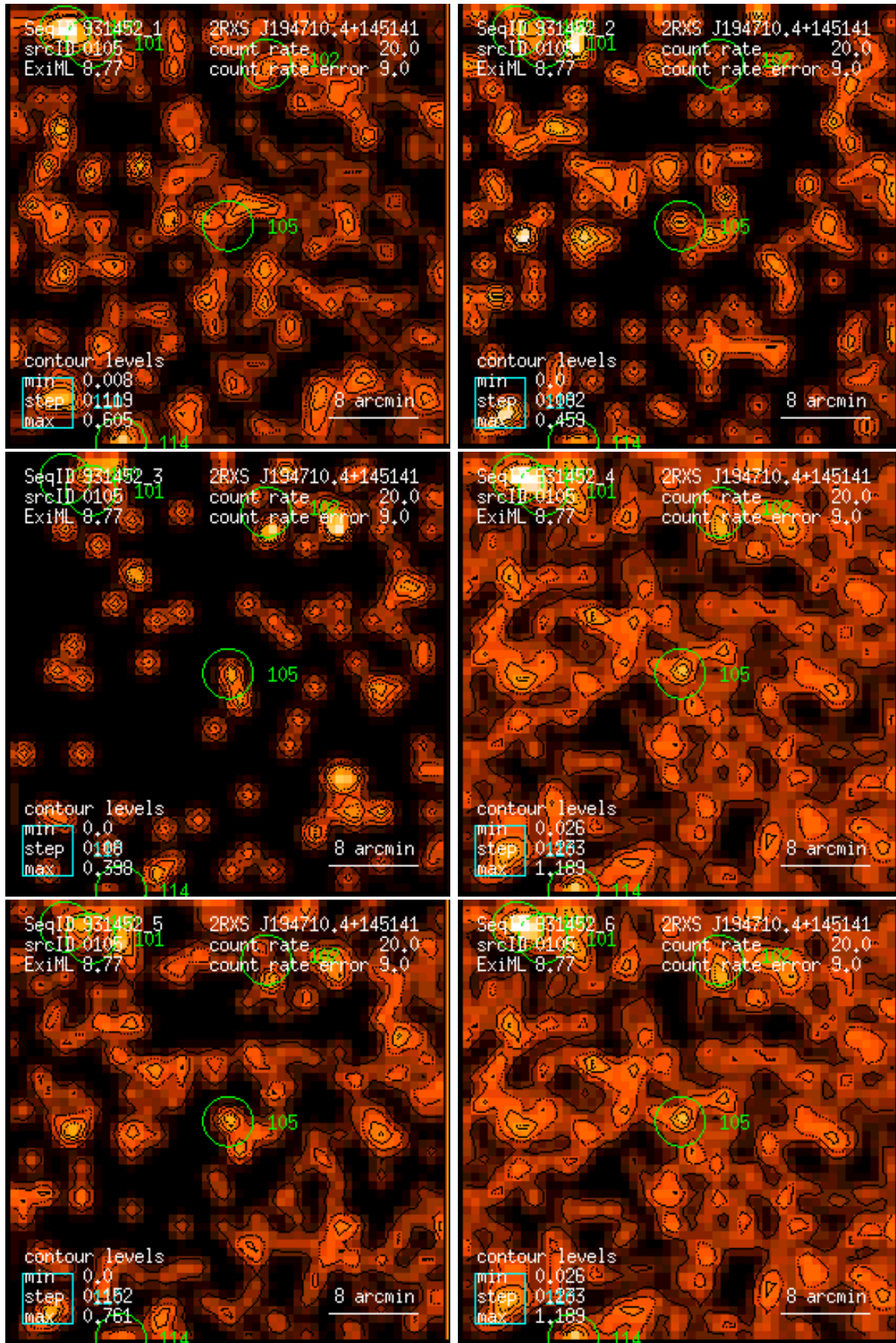
Figure 105: RASS 931452: detection 0105: band rate images, Gaussian filter: (1) PSPC channels 11 – 41, (2) 52 – 90, (3) 91 – 201, (4) 11 – 235, (5) 52 – 201, (6) 11 – 201. Broad band rates in counts/ks. Band rate contour levels in counts/ks/arcmin 2 .
