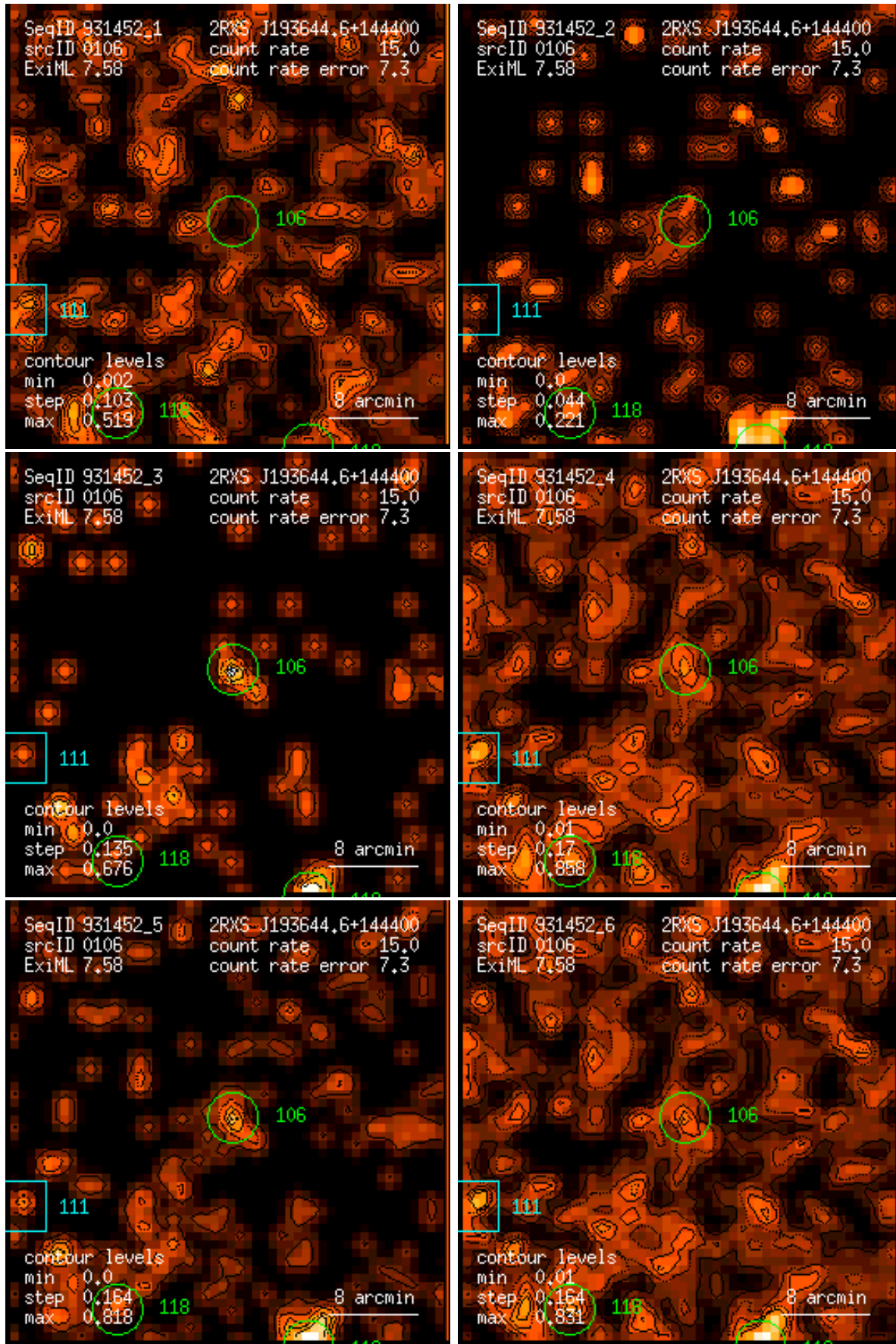
Figure 106: RASS 931452: detection 0106: band rate images, Gaussian filter: (1) PSPC channels 11 – 41, (2) 52 – 90, (3) 91 – 201, (4) 11 – 235, (5) 52 – 201, (6) 11 – 201. Broad band rates in counts/ks. Band rate contour levels in counts/ks/arcmin 2 .
