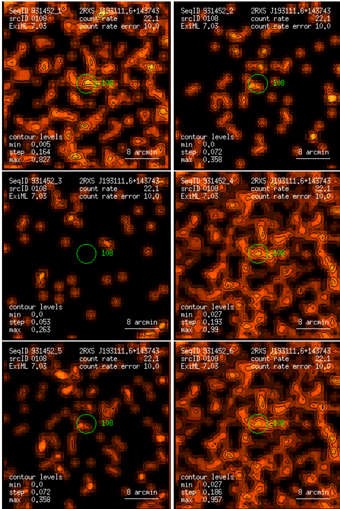
Figure 108: RASS 931452: detection 0108: band rate images, Gaussian filter: (1) PSPC channels 11 – 41, (2) 52 – 90, (3) 91 – 201, (4) 11 – 235, (5) 52 – 201, (6) 11 – 201. Broad band rates in counts/ks. Band rate contour levels in counts/ks/arcmin 2 .
