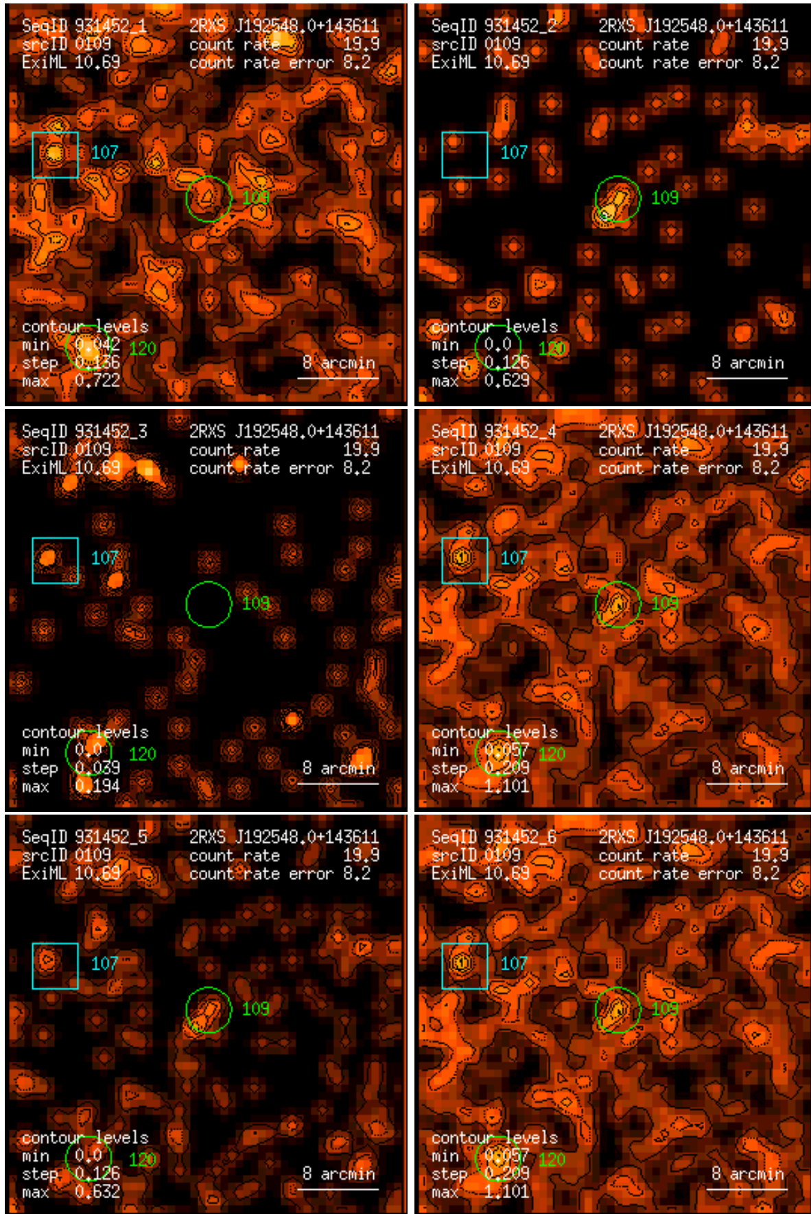
Figure 109: RASS 931452: detection 0109: band rate images, Gaussian filter: (1) PSPC channels 11 – 41, (2) 52 – 90, (3) 91 – 201, (4) 11 – 235, (5) 52 – 201, (6) 11 – 201. Broad band rates in counts/ks. Band rate contour levels in counts/ks/arcmin 2 .
