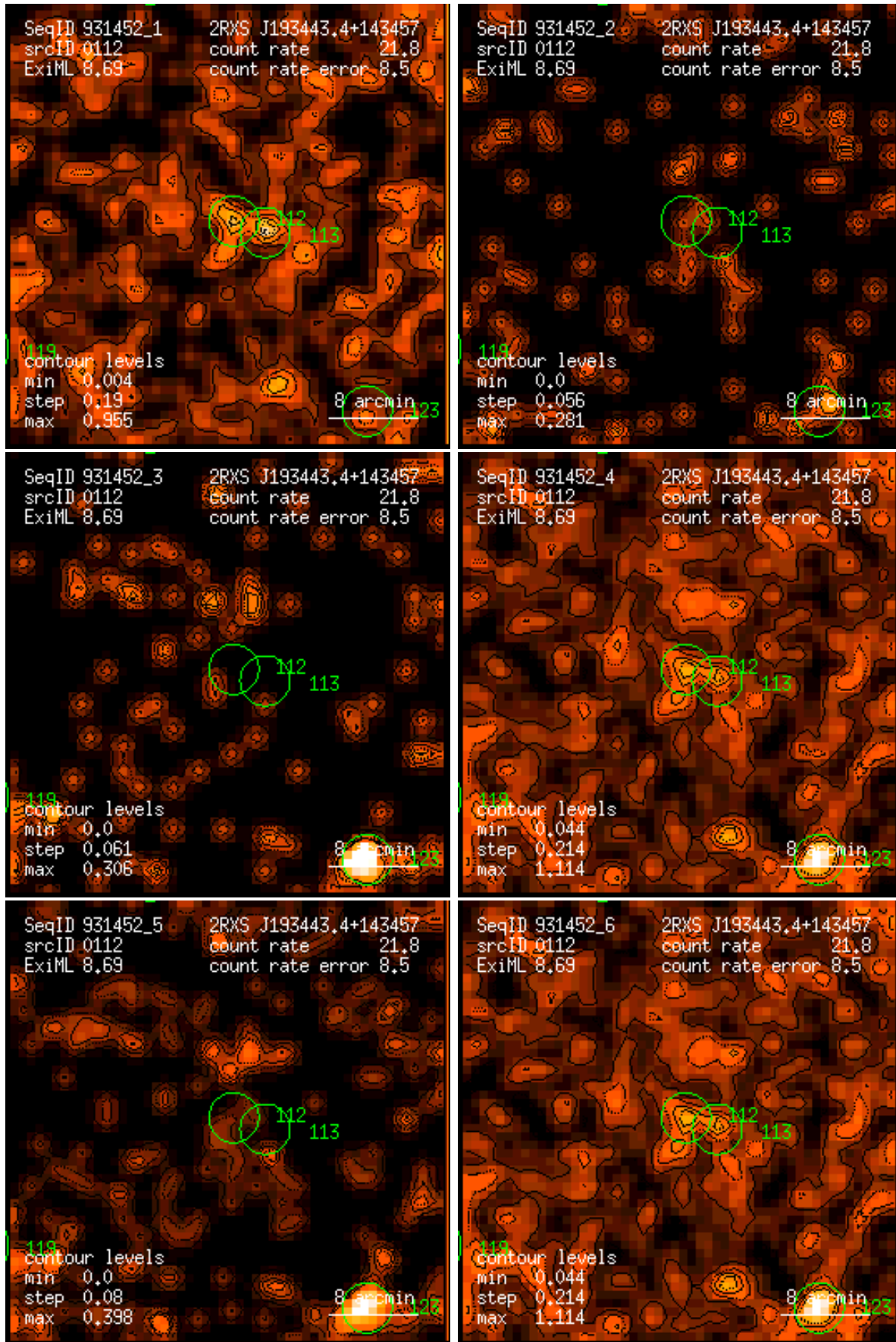
Figure 112: RASS 931452: detection 0112: band rate images, Gaussian filter: (1) PSPC channels 11 – 41, (2) 52 – 90, (3) 91 – 201, (4) 11 – 235, (5) 52 – 201, (6) 11 – 201. Broad band rates in counts/ks. Band rate contour levels in counts/ks/arcmin 2 .
