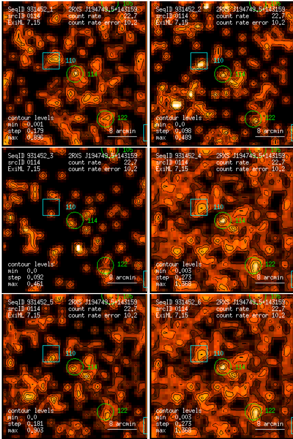
Figure 114: RASS 931452: detection 0114: band rate images, Gaussian filter: (1) PSPC channels 11 – 41, (2) 52 – 90, (3) 91 – 201, (4) 11 – 235, (5) 52 – 201, (6) 11 – 201. Broad band rates in counts/ks. Band rate contour levels in counts/ks/arcmin 2 .
